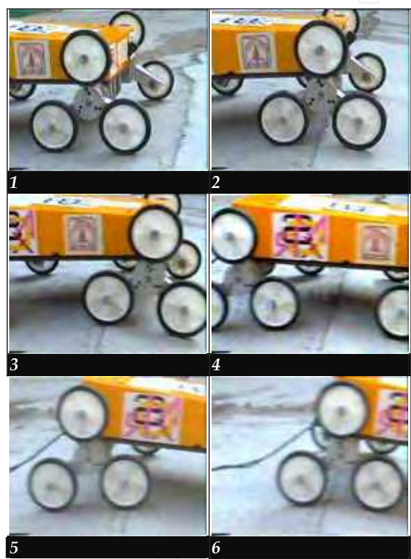
Figure 23. The MSRox adaptability in practice
