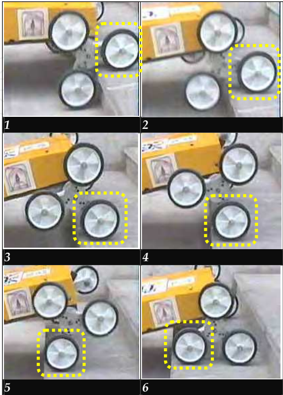
Figure 21. Similarity of Star-Wheels and human legs in practice According to the above figures the specified wheel has not any rotation and acts as a fixed base for MSRox. The MSRox Motion Adaptability While the robot moves on flat, uphill, downhill or slope surfaces, the star-wheels can rotate freely around their axes, that causes the robot adapts itself with respect to the curvature of the path. This adaptability also prevents the shocks that may be caused by the changes of surfaces slope. Also it keeps all 8 regular wheels in contact to the ground and prevents the separation of the regular wheels and the ground.
