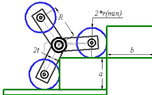
Figure 4. Star-Wheel Parameters
