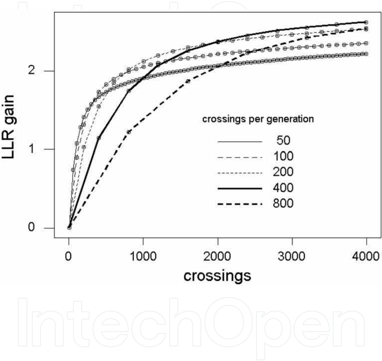
Figure 2. A numerical experiment shows how the number of well succeeded crossings per generation ( wsc_{MAX} ) affects the LLR gain. Each little square, representing one generation, consists of the average of 5,000 runs of the genetic algorithm. A total of 4,000 well succeeded crossings were simulated for each run, for several values of wsc_{MAX} . In a given curve, with a fixed number of crossings per generation, the LLR value increases rapidly at the beginning, slowing further in the next generations. The optimal value for wsc_{MAX} is 400, in this case. Had the total of well-succeeded crossings been 1,000, the optimal value of wsc_{MAX} should be 200, as may be seen placing a vertical line at the 1,000 position.
