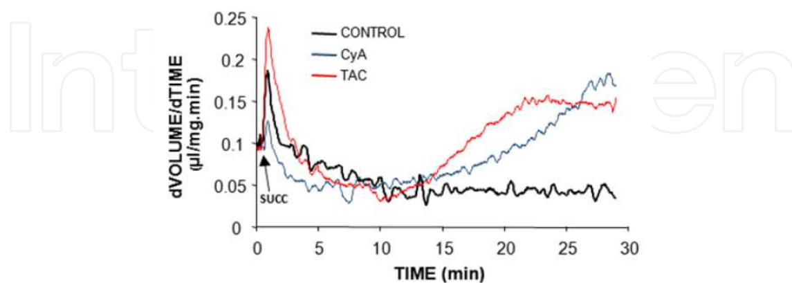
Figure 10. Early and delayed mitochondrial permeability transition pore opening by cyclosporin A (CyA) and tacrolimus (TAC). Incubation of a mitochondrial solution with 1 μg/mL CyA or 50 ng/mL TAC during at least 30 minutes produced a second increase in mitochondrial volume. Succinate-induced mitochondrial swelling was determined spectrophotometrically at 520 nm.
