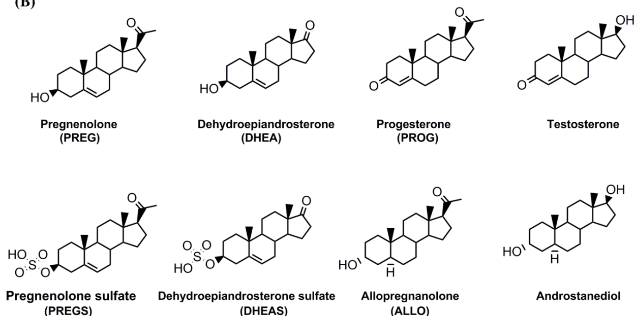
Figure 3. Chemical structure of cholesterol and neurosteroids. Cholesterol (A) is converted into various neurosteroids (B). Each neurosteroid has significant roles in the brain and nerve system, but these neurosteroids, specifically, have shown neuroprotective properties.
