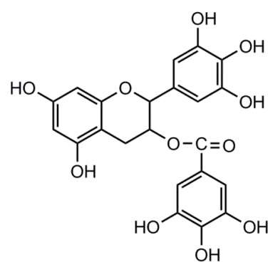
Epigallocatechin gallate (EGCG)
