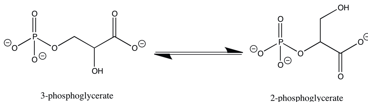
Figure 14. Enzymatic reaction for phosphoglycerate mutase.
