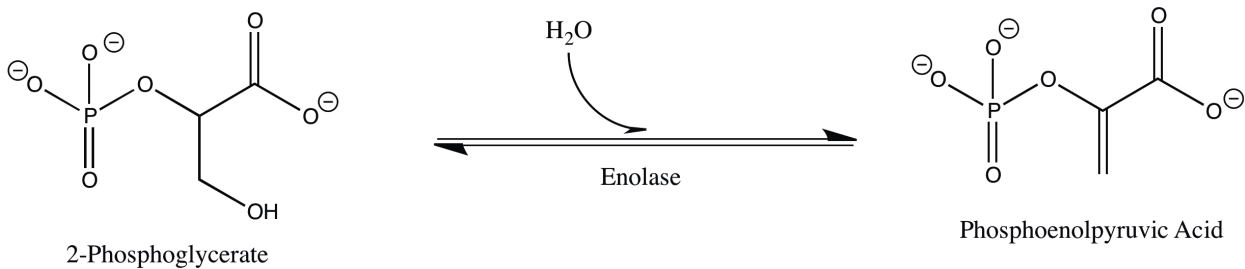
Figure 12. Enzymatic reaction for enolase.
