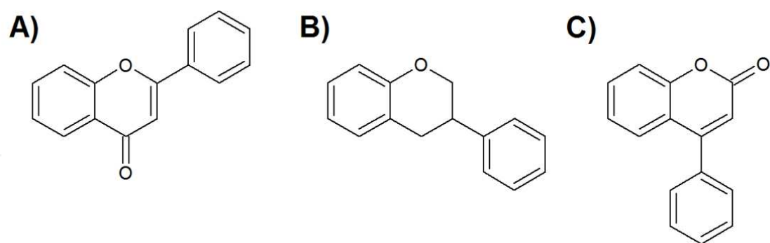
Figure 4. The flavone (A), isoflavan (B), and neoflavonoid (C) structures serve as the chemical backbones for flavonoid compounds.
