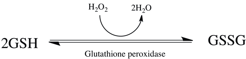
Glutathione peroxidase enzyme reaction
