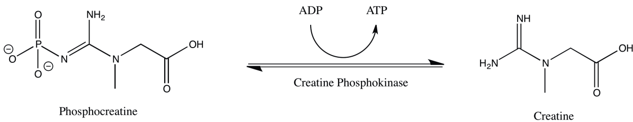
Figure 13. Enzymatic reaction for creatine kinase.
