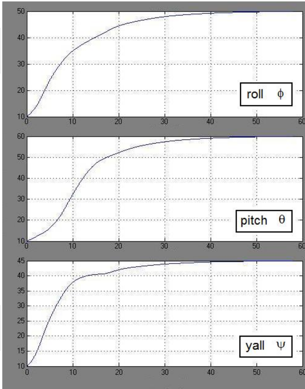
Figure 8. Co-simulation results of attitude control for the three Euler's angles, considering a tracking maneuver.
