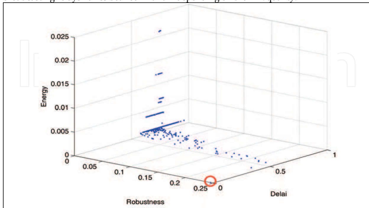
Fig.12. Estimated Pareto front for the single communication performance estimation problem
