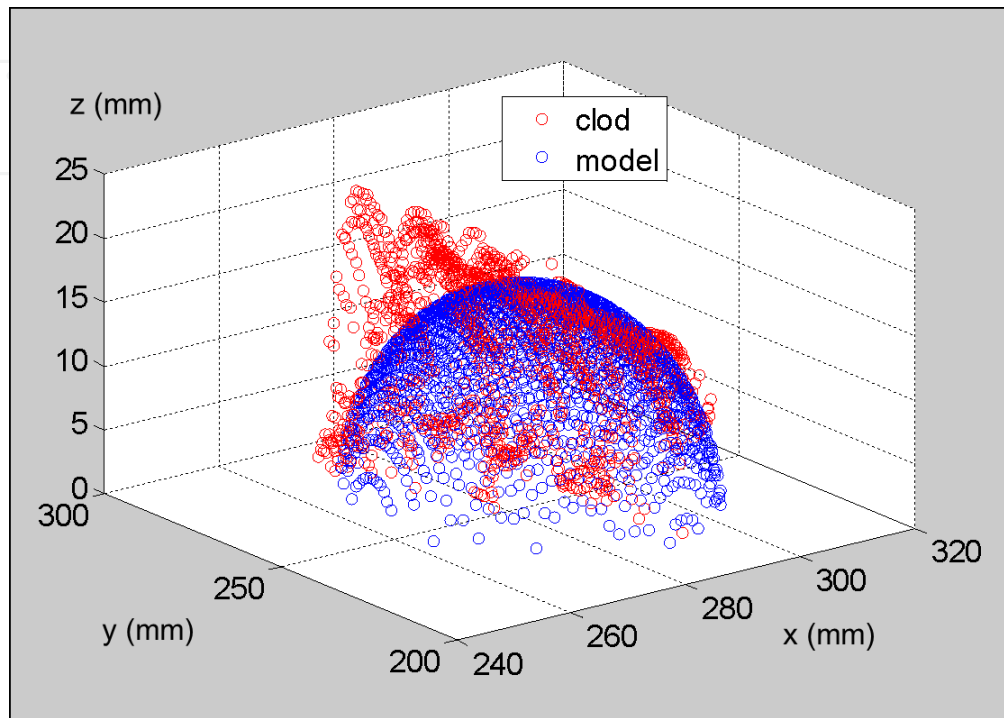
Figure 6. Clod modelling by a half ellipsoid
