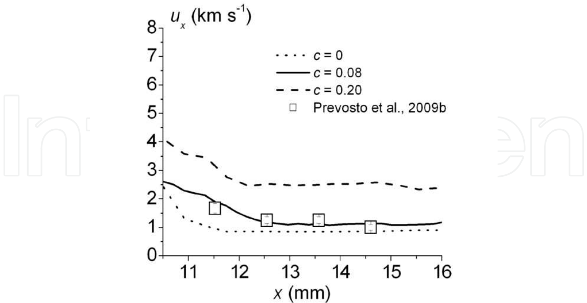
Figure 7. Averaged theoretical axial plasma velocity over the emitting arc cross section, defined from the arc core (axis) to the \approx 4000 K temperature line for the same c values presented in Fig. 3. The experimental values corresponding to an averaged emission over the whole emitting section of the arc are also shown. Taken from Mancinelli et al., 2011.
