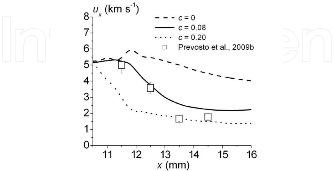
Figure 6. Comparison between calculated plasma velocity values at the axis for c = 0 , c = 0.08 and c = 0.20 , and the measured values of the axial velocity corresponding to light emitted from the arc central core. Taken from Mancinelli et al., 2011.
