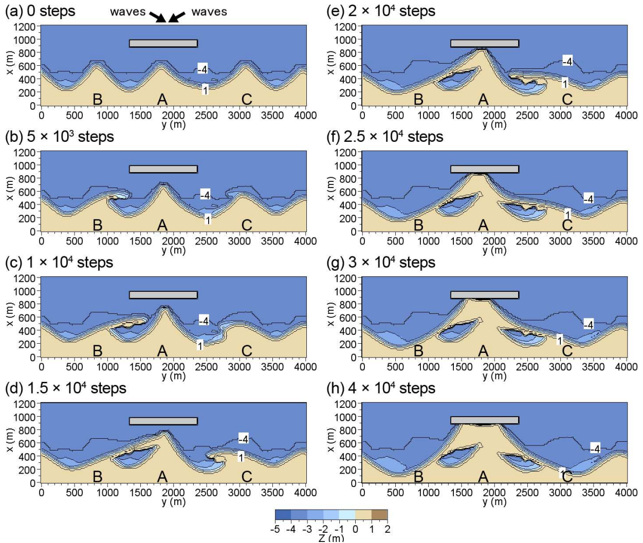
Figure 17. Deformation of cusplate forelands formed under the condition of oblique wave incidence from \pm 60^\circ with probabilities of 0.5:0.5 after construction of a breakwater offshore of apex of cusplate foreland A.
