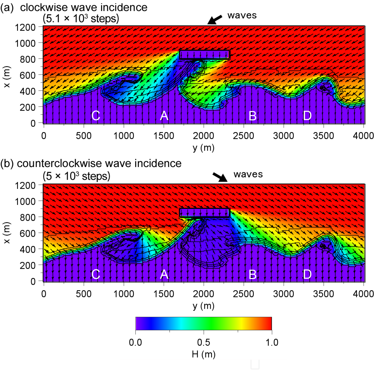
Figure 21. Wave field around a breakwater after 5.1 \times 10^3 and 5 \times 10^3 steps.
