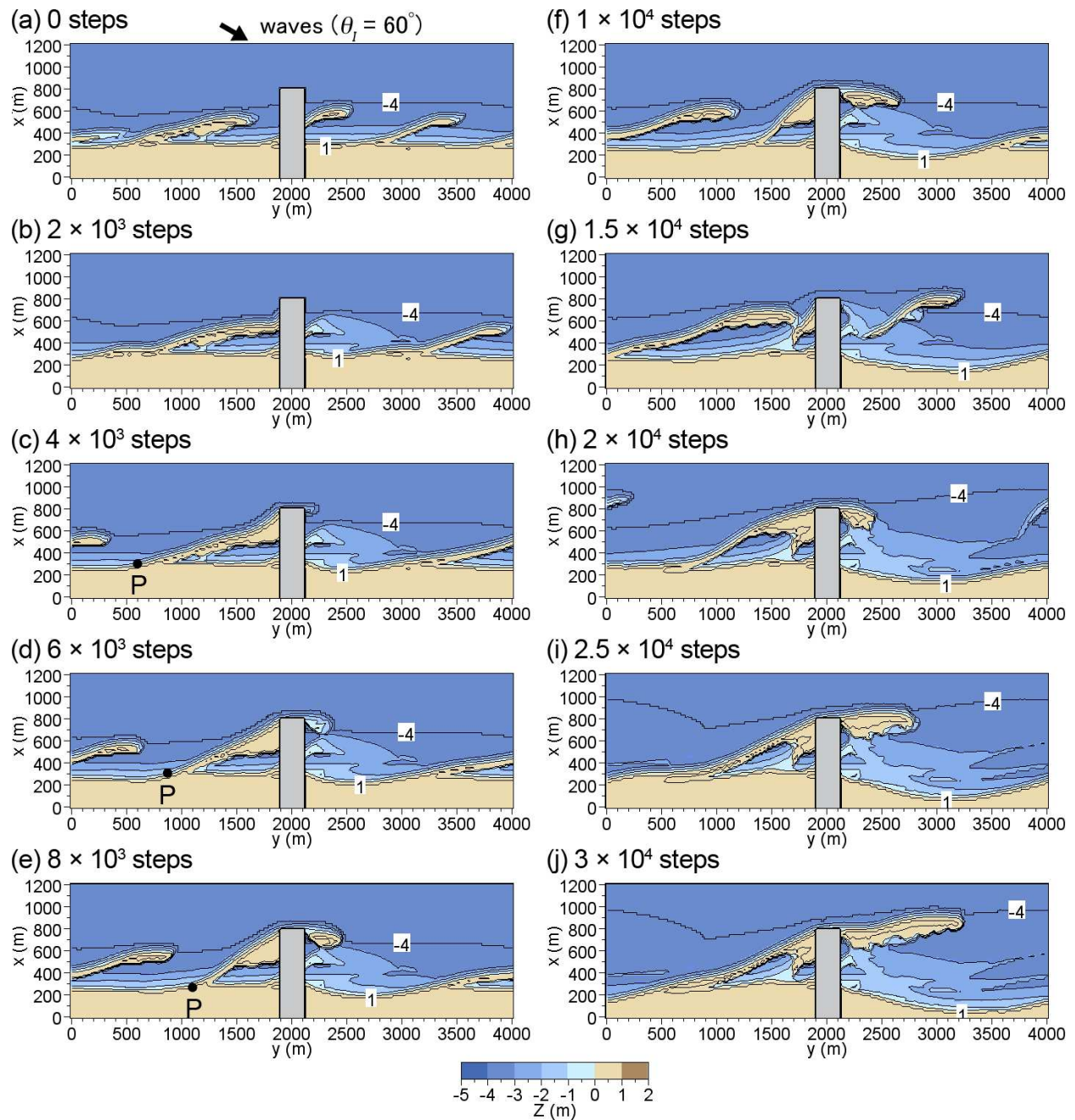
Figure 14. Deformation of sand spits formed under oblique wave incidence from 60° after extension of a groin.
