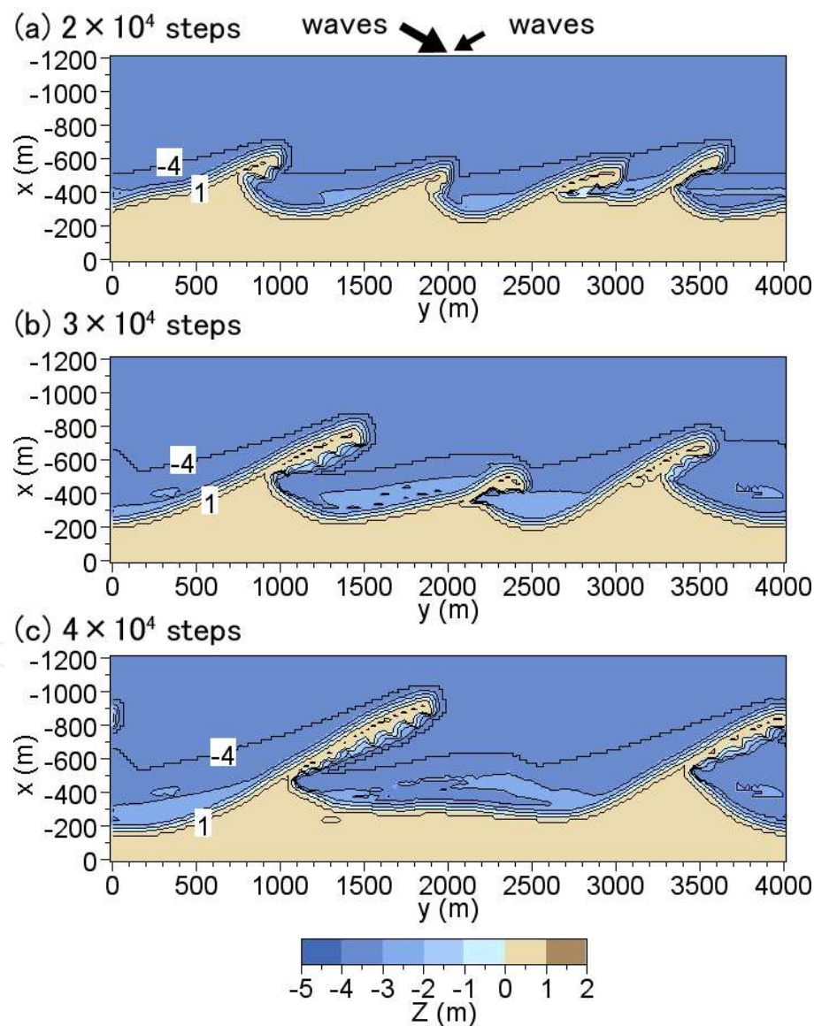
Figure 11. Formation of cusped forelands (oblique wave incidence from \pm 60^\circ with probabilities of 0.70:0.30).
