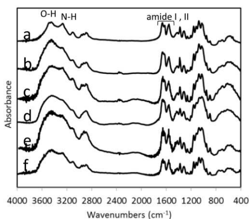
Figure 10. FT-IR spectra of a) commercial chitin, and CNFs from mushroom source of species b) Lentinula edodes , c) Pleurotus eryngii , d) Hypsizygus marmoreus , e) Grifola frondos , and f) Agaricus bisporus . Reprinted from ref. 3.
