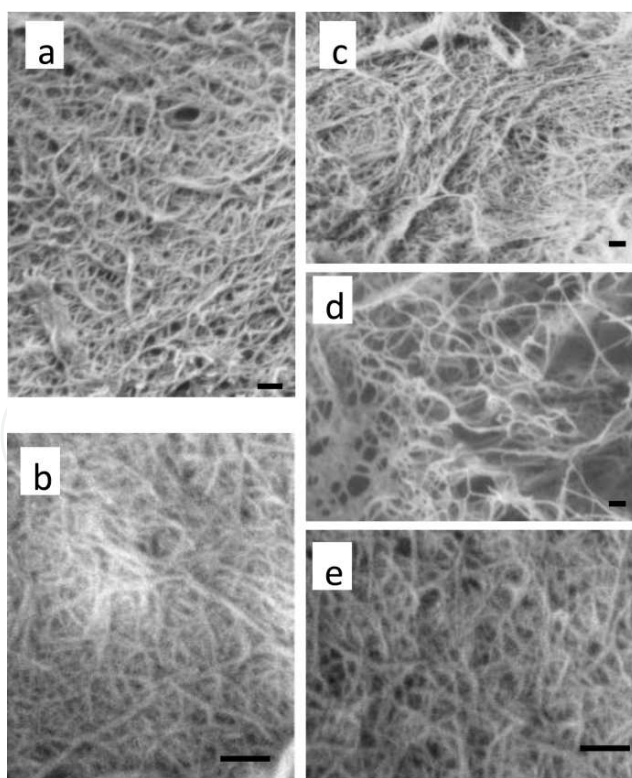
Figure 9. FE-SEM images of CNFs prepared from a) Pleuotus eryngii , b) Agaricus bisporus , c) Lentinula edodes , d) Grifola frondosa , e) Hypsizygus marmoreus . The scale bars are 200 nm. Reprinted from ref. 3.
