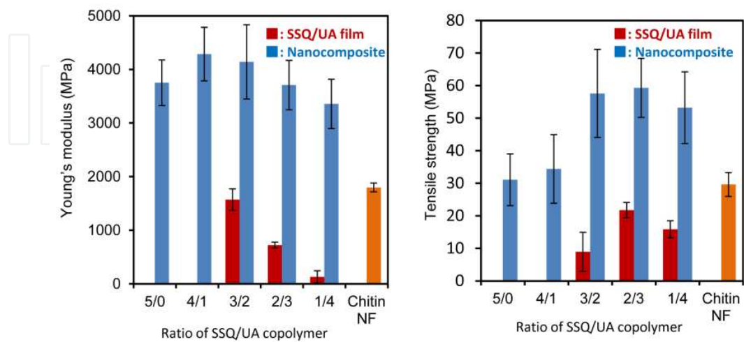
Figure 15. Young’s modulus and tensile strength of SSQ-UA copolymer and SSQ-UA-CNFs composites. Reproduced with permission from ref. 6. Copyright 2012, Elsevier.
