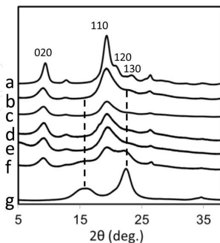
Figure 11. XRD pattern of a) commercial chitin, and CNFs from mushroom source of species b) Pleurotus eryngii , c) Agaricus bisporus , d) Lentinula edodes , e) Grifola frondos , f) Hypsizygus marmoreus , and g) commercially available cellulose. Reprinted from ref. 3.
