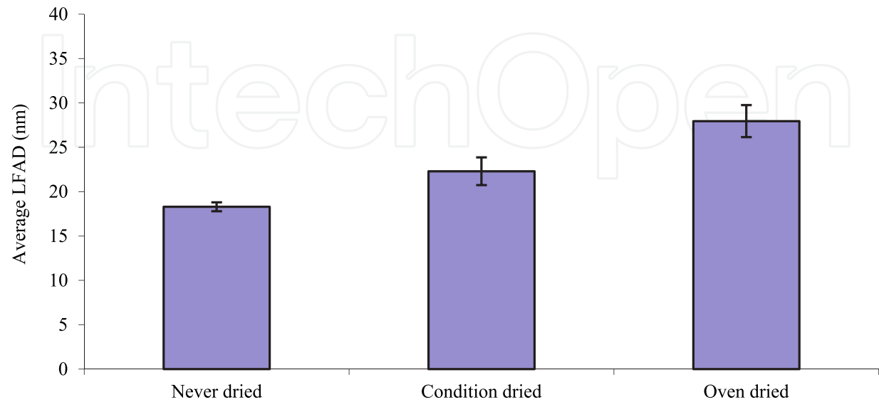
Figure 6. Average LFAD (nm) for the '92% α-cellulose' using the different drying strategies
