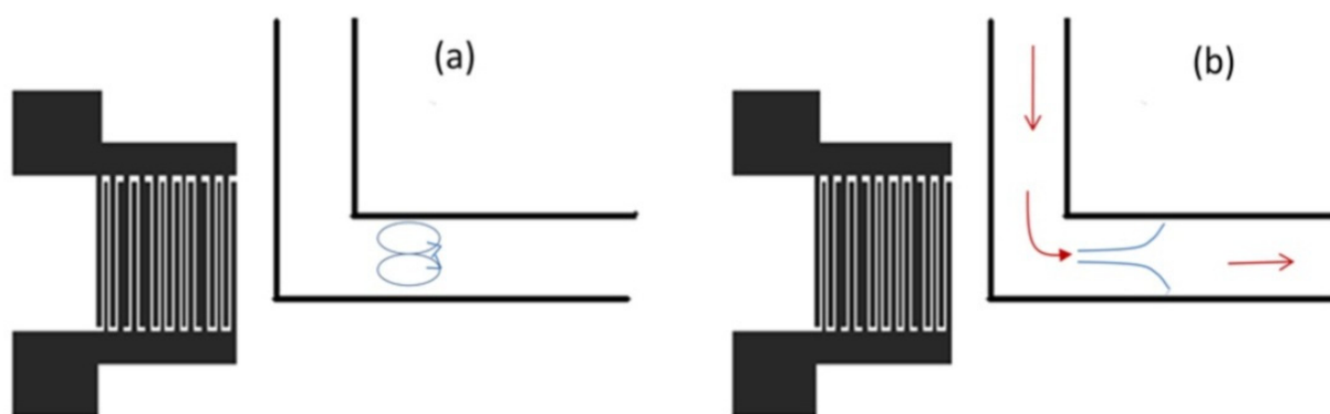
Figure 18. Principle of SAW-based micropumps with a channel. When the vortex is smaller than the channel width, the back flow occurs, suitable for in-channel mixing (a). When the vortex is larger than the channel width, a unidirectional flow is formed (b).
