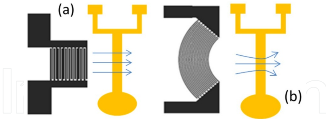
Figure 19. Schematic drawing of SAW-based in-channel micromixer.
