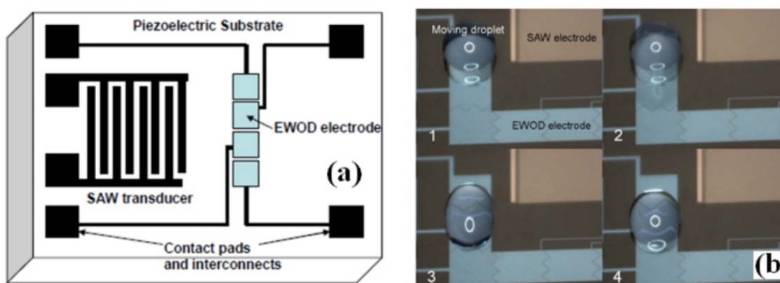
Figure 23. Schematic of integrated EWOD and SAW test structure and the droplet generation by EW and manipulation by SAW [82]. Reprinted with permission from AIP, Biomicrofluidics, 6, 2012, 012812.
