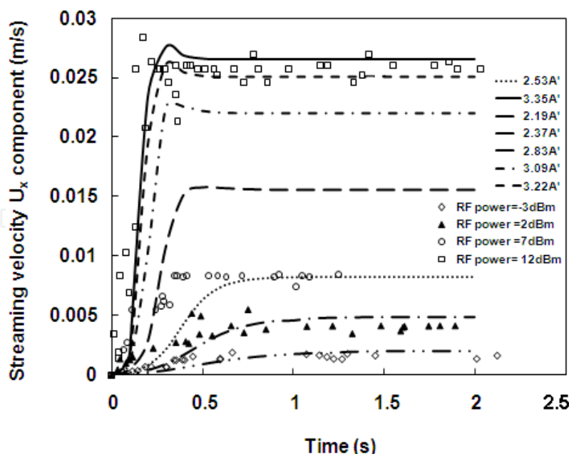
Figure 8. Streaming velocity at top centre of a 30 \mu\text{l} droplet. SAW device has f=62\text{MHz} , an aperture of 2mm; Solid lines represent numerical results at different wave amplitudes; the symbols are experimentally measured data at different RF powers [53]. Reprinted with permission from Institute of Physics, J. Microeng. Micromech. 21, 2011, 015005.
