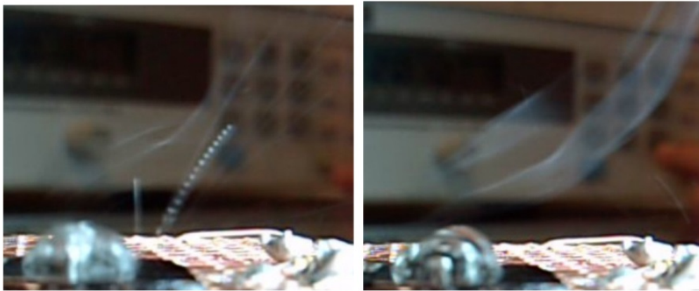
Figure 24. Acoustic streaming induced mist by a ZnO SAW device, which may reach 6mm height.
