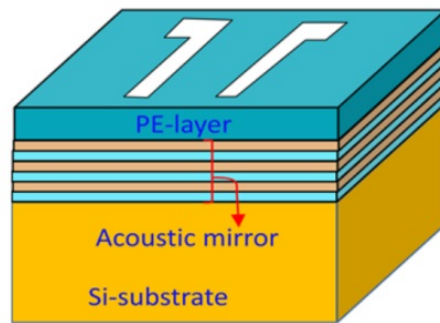
Figure 29. Schematic structure for the lateral field excited FBAR devices, which generates a thickness shear mode resonance.
