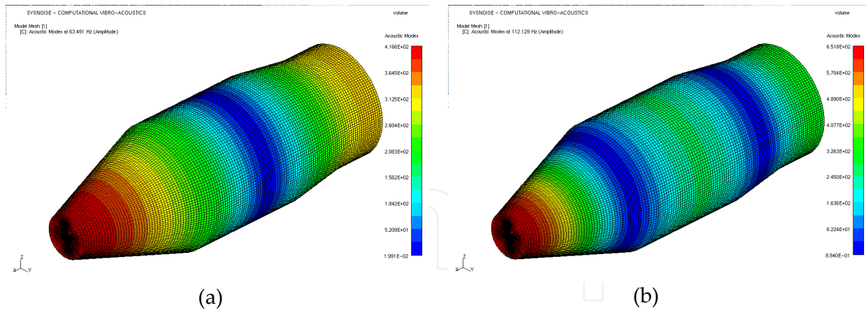
Figure 10. a) First acoustic longitudinal mode; b) Second acoustic longitudinal mode
