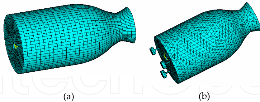
Figure 22. a) Cavity without resonators; b) Cavity with resonators
