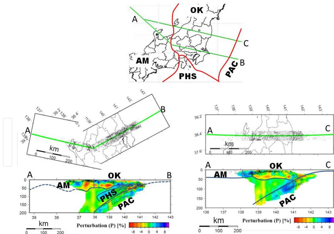
Figure 6. P-wave perturbation structures beneath the central Japan. This section image obtained by high-density seismic stations by seismic tomography using a viewer software developed by NIED to estimate the 3D seismic velocity structure typical of under Japan. Data are quoted from [73]. Tohoku and Seinan arcs are distinctive in rheology structure due to difference in plate configuration.
