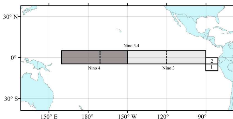
Figure 3. Pacific Ocean and corresponding Nino regions
