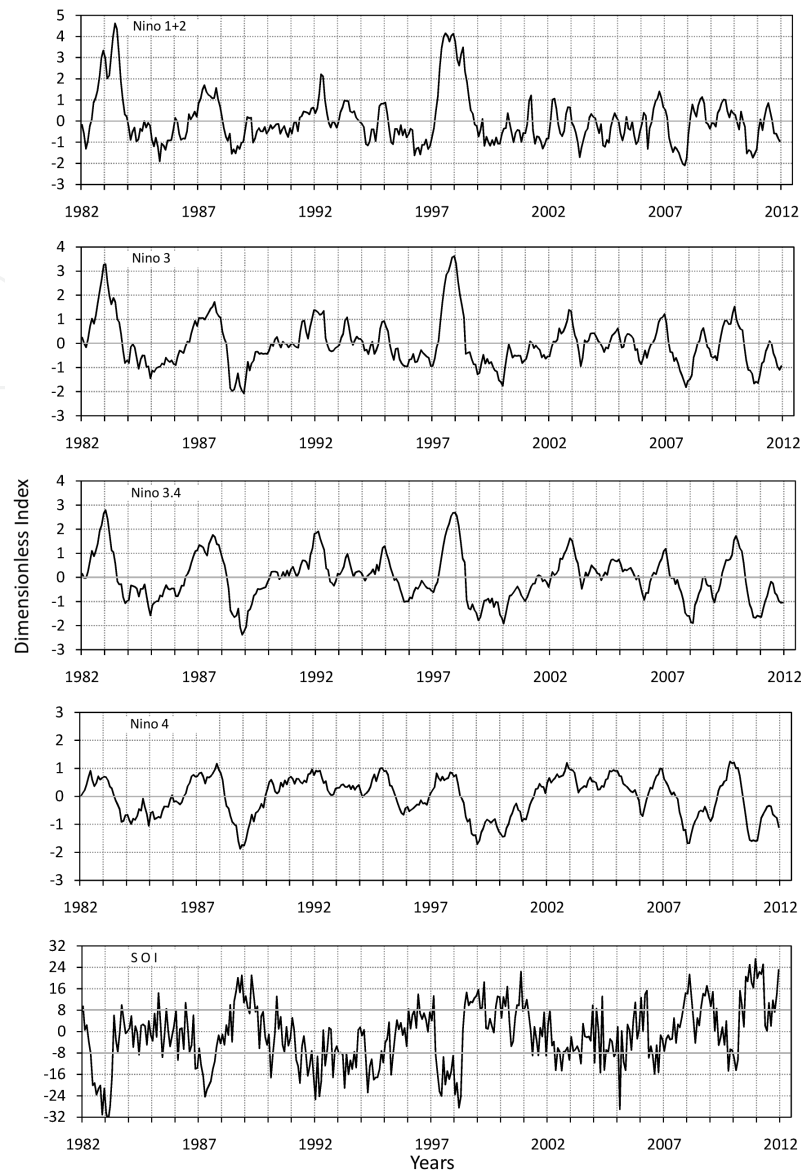
Figure 4. Fluctuation of ENSO indices monthly values during 1982-2011
