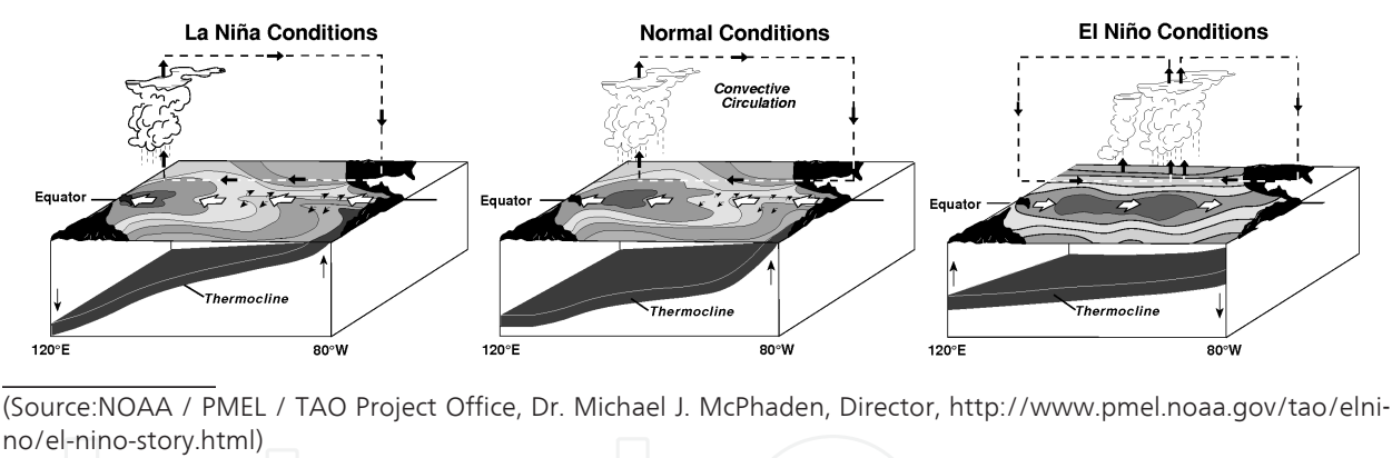
Figure 1. Schematic diagram of ENSO climate pattern in the Pacific Ocean
