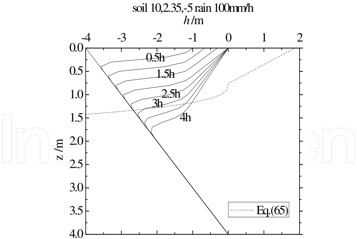
Figure 42. Infiltration results without air phase consideration
