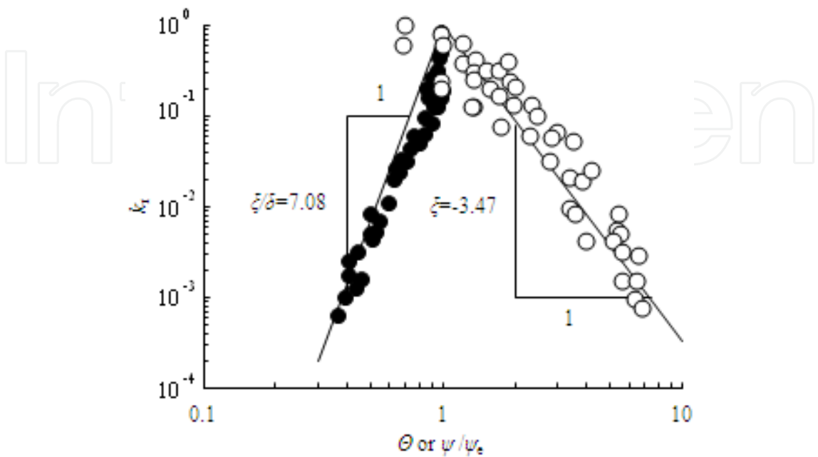
Figure 27. Comparisons between predictions and experimental data of RHC for McGee Ranch soil (Data from Hunt and Gee, 2002)
