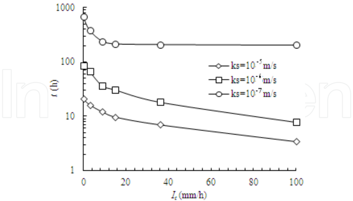
Figure 41. The time of failure vs. rainfall intensity
