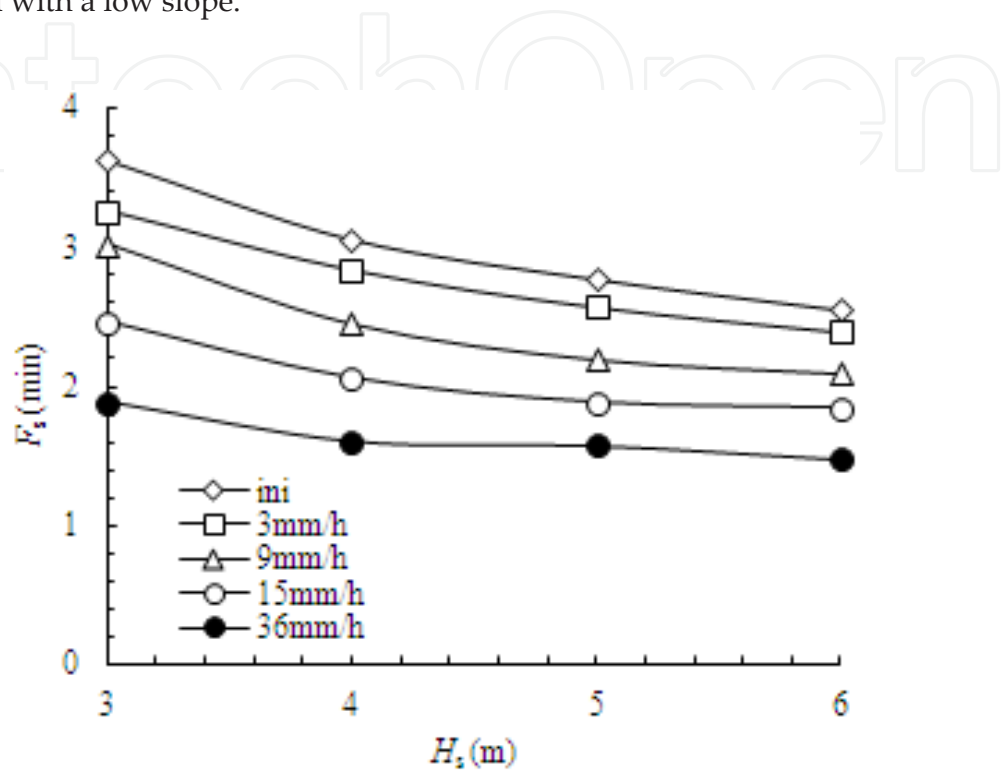
Figure 50. Effect of slope height on factor of safety
