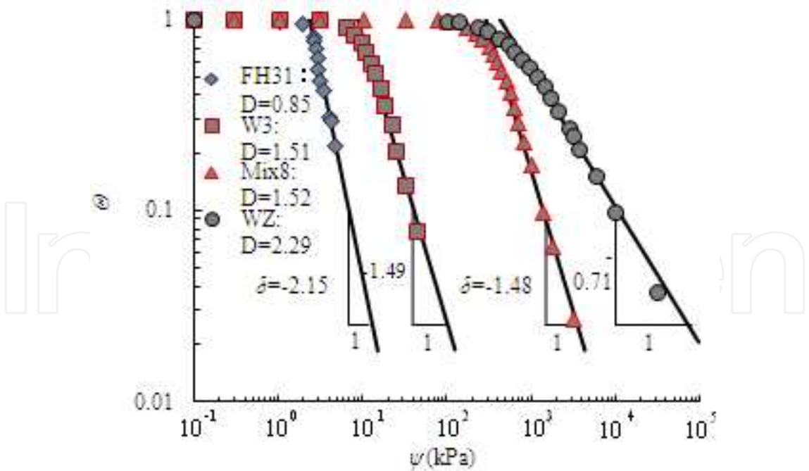
Figure 16. Comparison between the predictions of Eq. (29) and experimental data of SWCCs (Data from Stingaciu et al. 2009)
