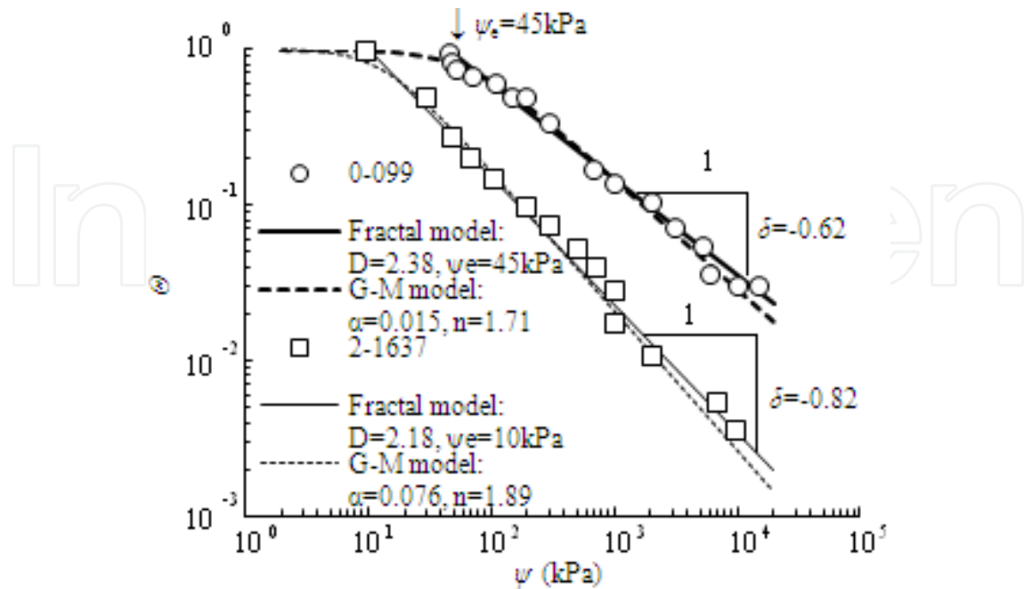
Figure 30. Fractal dimension and G-M parameters obtained from SWCC for Hanford glacial (Khaleel and Relyea, 1995)
