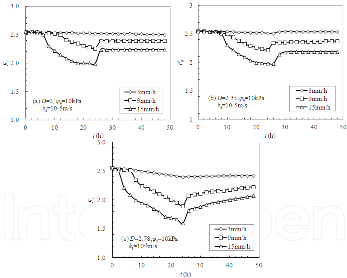
Figure 44. Effect of fractal dimension on slope stability
