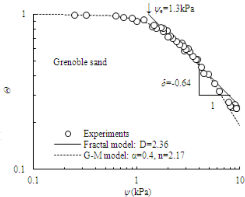
Figure 32. Fitted SWCC curves
