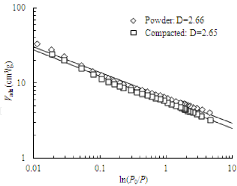
Figure 6. The surface fractal dimension of Tsukinuno bentonite from nitrogen adsorption
