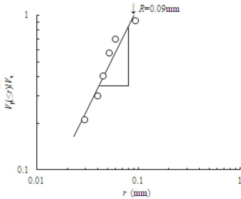
Figure 5. The fractal dimension and the maximum radius evaluated from the PSD of Toyoura sand. (Data from Uno et al., 1998.)
