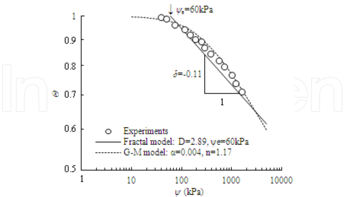
Figure 28. Fractal dimension and the parameters of G-M model obtained from SWCC for Beit Netofa clay (Data from van Genuchten, 1980)
