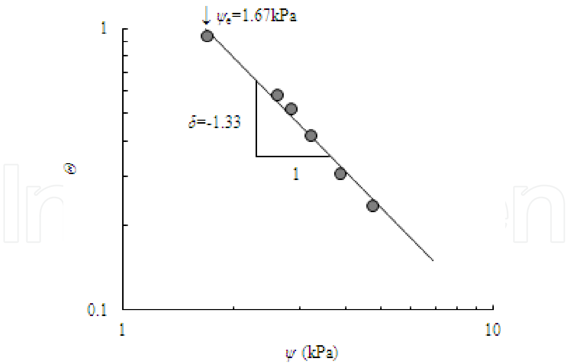
Figure 14. Comparison of the SWCCs for Toyoura sand (Data from Uno et al., 1998)
