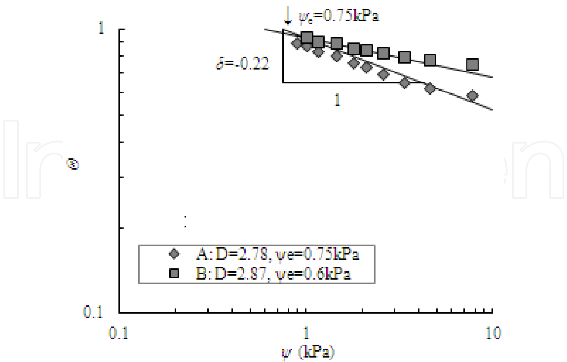
Figure 13. Comparison between prediction and experiments of SWCCs (Data from Vogel and Roth, 1996)
