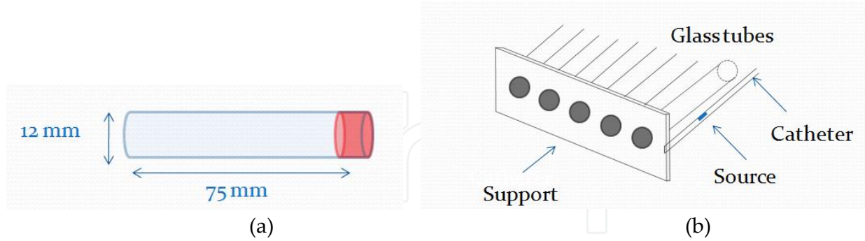
Figure 4. (a) Glass tube of 5 ml and (b) scheme of the setup to determine the calibration curve for the gel dosimeter.
