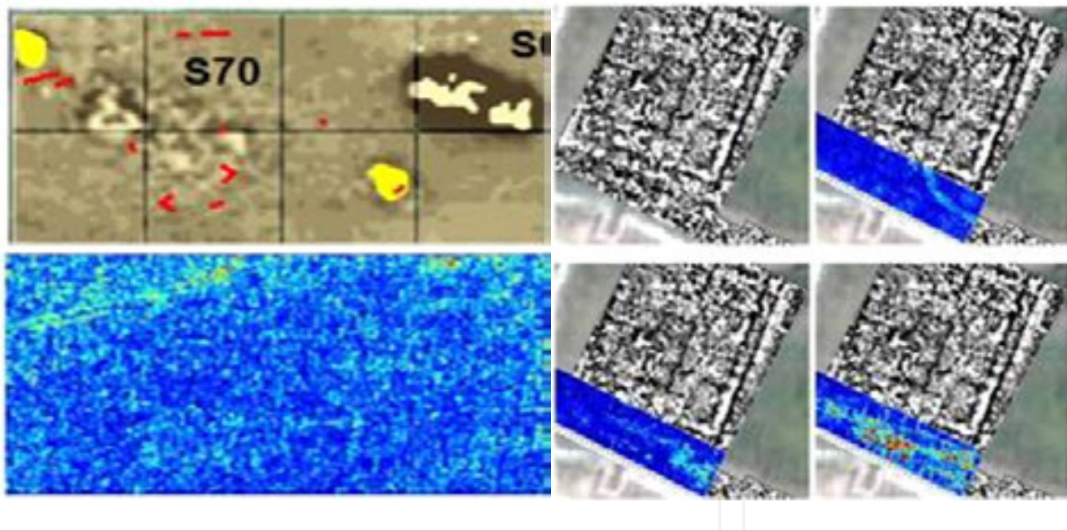
Figure 25. Left: Comparison between magnetic and GPR prospection above structural remains of the flat settlement at Szeghalom site in East Hungary. Even though the foundations of the daub constructions are registered clearly to the magnetic data (left top), the high conductivity of the soils has attenuated strongly the GPR electromagnetic signals masking completely the particular area (left bottom) (Sarris 2012). Right: Comparison between magnetic and GPR prospection at the corner of the Palaeochristian fortifications of Nikopolis, Epirus (Greece). The color maps represent the GPR horizontal slices of 0.1m width for depths of 0.5 (top right), 1 (bottom left) and 1.5m (bottom right) approximately. The remains of a structural complex are obvious in the magnetic data. The GPR managed to register reflectors originating from various depths, such as a curving path at the top layers and a section of decumanus maximus at the lower bottom of the surveyed area. The latter was not clearly resolved in the magnetic data as the high surface concentration of sherds created a uniform magnetic background masking of the area of interest.
