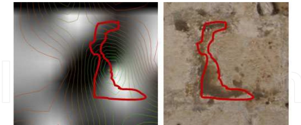
Figure 24. Visual comparison of the ultrasonic measurements and close range photographs. The polygons are drawn as common areas for each set of figures.
