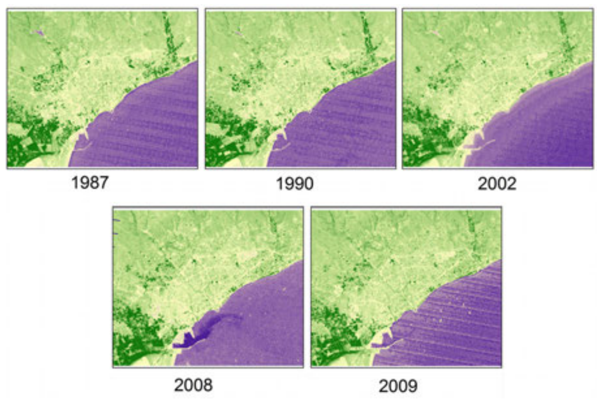
Figure 8. NDVI maps produced from Landsat dataset.
