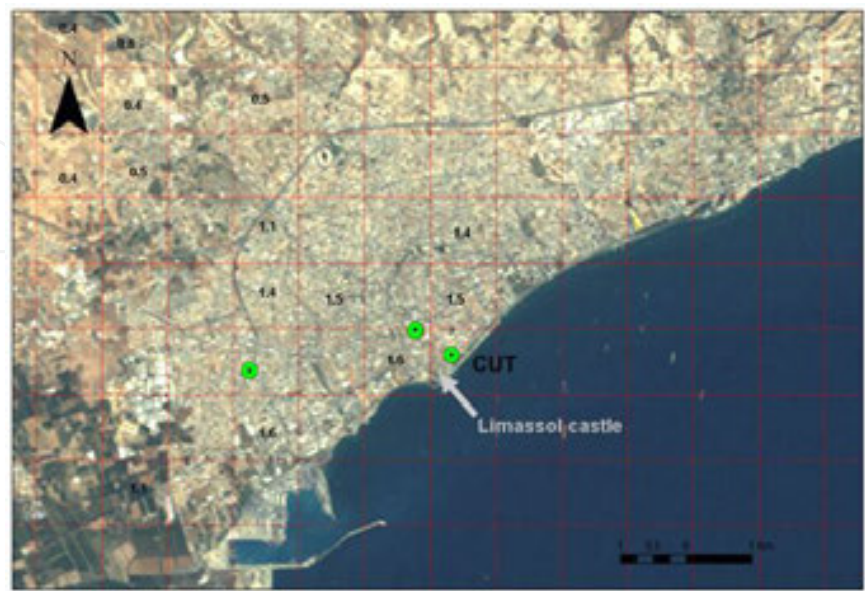
Figure 10. AOT levels in the Limassol area. High AOT levels are noted in the area near the Limassol Castle.
