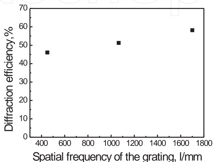
Figure 7. Diffraction efficiency of three gratings multiplexed in the same region of a photopolymer layer of thickness 120 \mu\text{m} .
