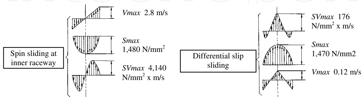
Figure 2. Sliding frictional conditions at inner and outer raceways for \text{LH}_2 bearing (25-mm bore, 50,000 rpm, 980 N)
