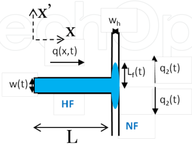
Figure 7. Illustration of the HF-NF interaction scheme in analytical model
