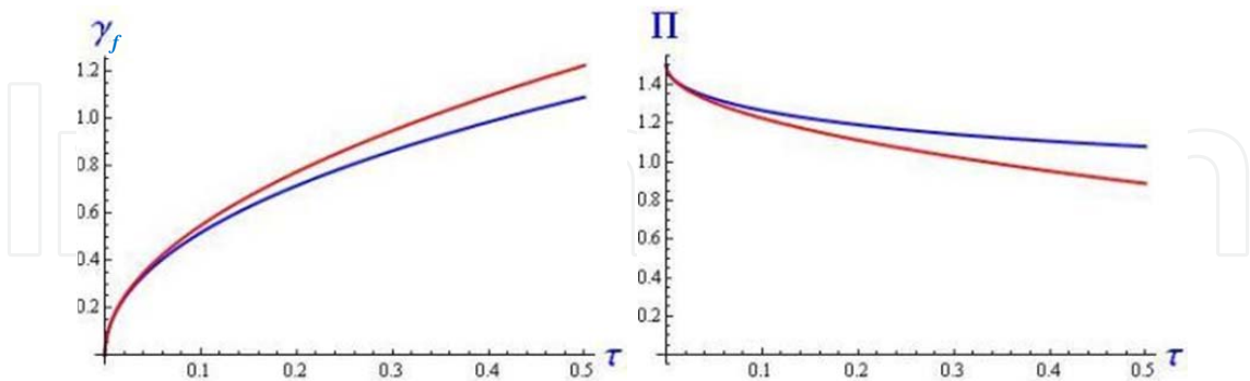
Figure 9. Asymptotic (red) and numerical (blue) solutions for the dimensionless fluid penetration length (left) and fluid pressure in junction point (right) at the early time of fracture contact
