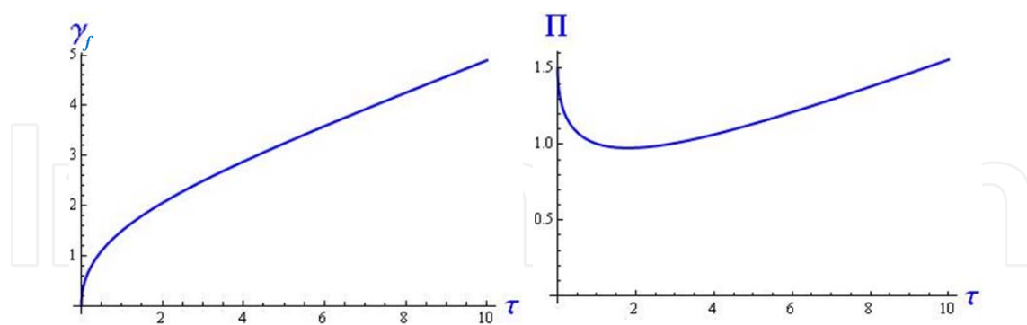
Figure 8. Analytical solution of the dimensionless problem for fluid penetration into NF (34) for dimensionless permeability \Psi_h = 1 , and initial pressure \Pi_{00} = 1.5 . Left plot is the dimensionless fluid front propagation along the NF in time. Right plot is the change of dimensionless pressure at the HF-NF intersection point.
