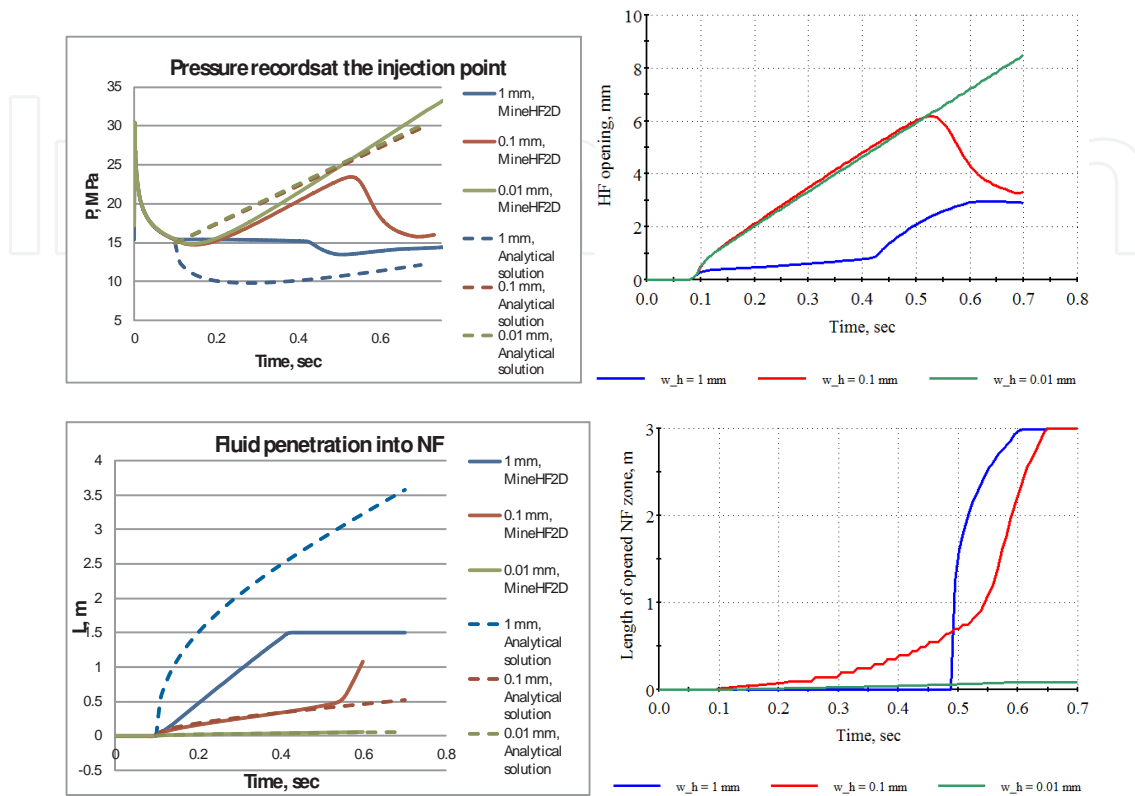
Figure 11. Results of numerical experiments with \kappa_{IC}=0.32 , \Sigma_2=0.8 , \Delta\Sigma=1 , \beta=90 , \lambda=0.2 and three values of residual hydraulic opening at the NF permeability (blue: 1 mm; red: 0.1 mm; green: 0.01 mm). Top left: fluid pressure changes at the inlet. Top right: opening of the HF at junction. Bottom left: fluid penetration length along the NF. Bottom right: total length of the mechanically open zone at the NF in meters.
