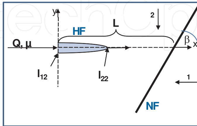
Figure 1. Schematic representation of the problem statement where a plain-strain (Khristianovich-Zheltov-DeClerk) model is considered with a one-wing HF is propagating toward a discontinuity (NF)
