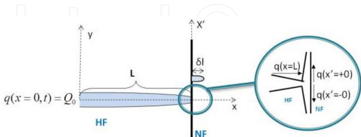
Figure 2. Boundary conditions of the problem
