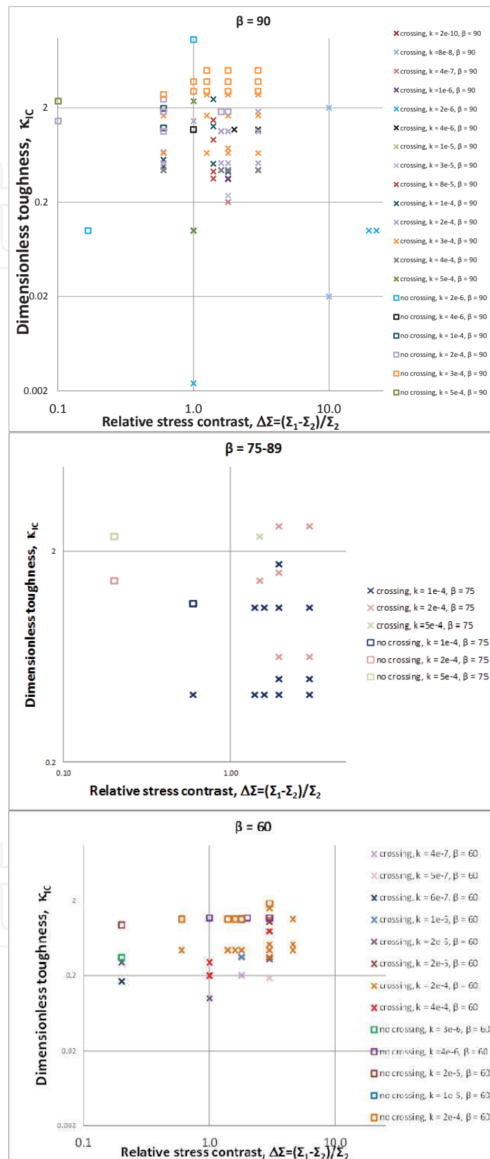
Figure 5. Crossing vs. arresting diagram in (\kappa_{IC}, \Delta\Sigma) for different angles of fracture interaction. \kappa_{IC}^{(NF)} = 0 .
