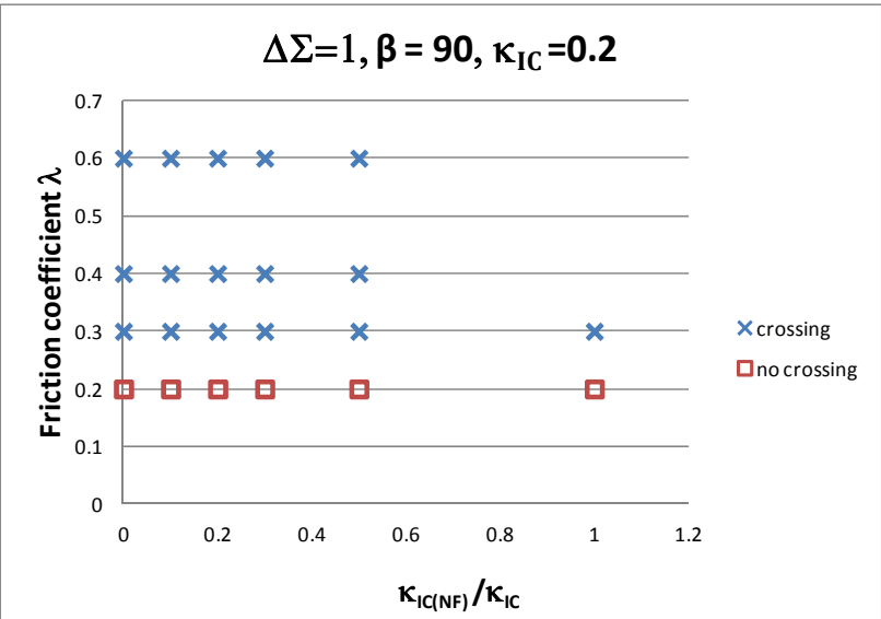
Figure 6. Crossing vs. arresting diagram in (\lambda, \kappa_{IC(NF)}/\kappa_{IC}) .
