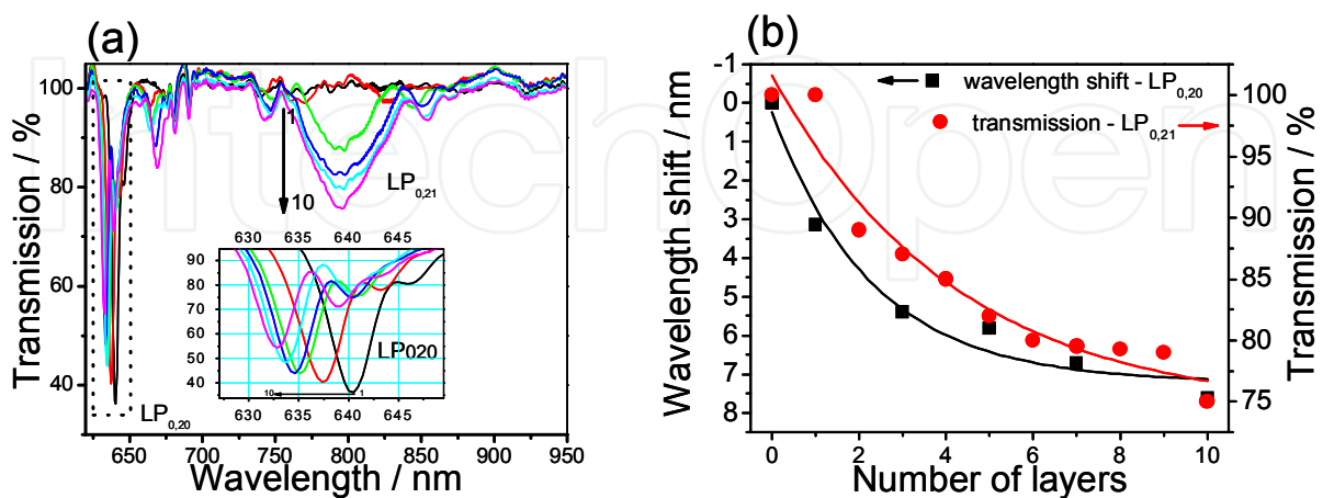
Figure 7. (a) Transmission spectra of the 100 \mu m period LPG in the colloidal SiO_2 solution in water after PDDA deposition (b) wavelength shifts and changes in transmission as a function of the number of deposition cycles for the LP_{020} and LP_{021} resonance bands, respectively; the curve is a guide to the eye only.
