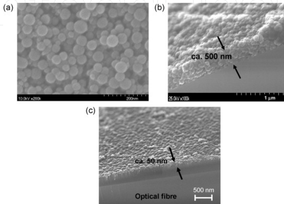
Figure 6. SEM images of the (a) surface morphology and (b) cross-section of the (PDDA/SiO_2)_{10} film deposited on a quartz substrate before TSPP infusion; (c) cross section of a (PDDA/SiO_2)_1 film.
