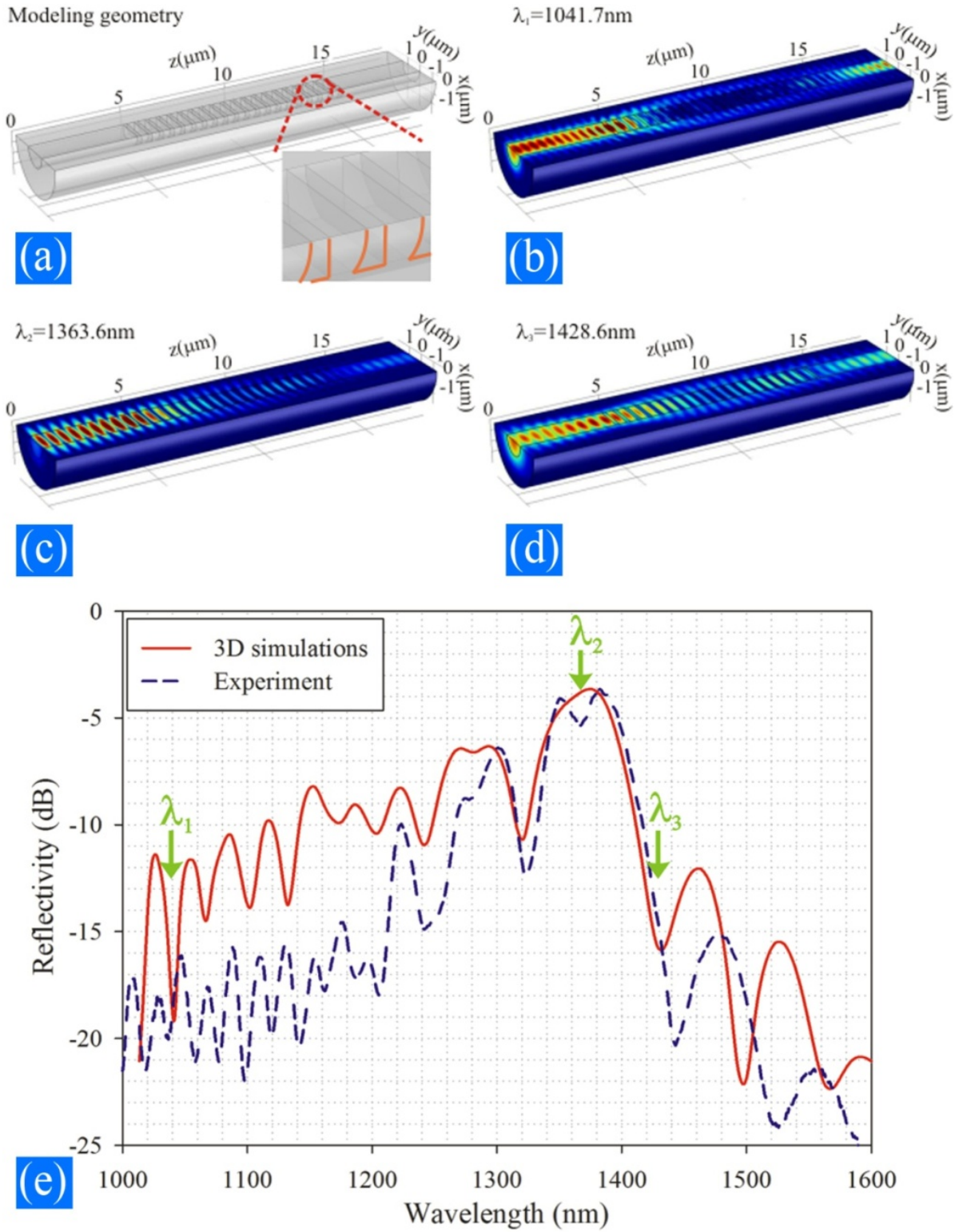
Figure 3. (a) Schematic of a 3D finite element simulation of SCMG; the insert shows the magnified figure of the biconcave air notch. (b), (c), and (d) Electric fields at wavelengths \lambda_1 = 1041.7\text{nm} , \lambda_2 = 1363.6\text{nm} , and \lambda_3 = 1428.6\text{nm} , respectively. (e) SCMG reflection spectra. The red solid line is the 3D simulation line while the blue dashed line is the experiment result. \lambda_1 , \lambda_2 , and \lambda_3 represent the wavelengths whose electric fields are shown in (b), (c), and (d) [19].
