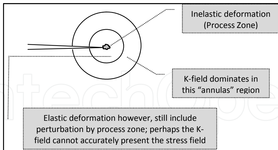
Figure 2. Process zone and K-field representation [3]
