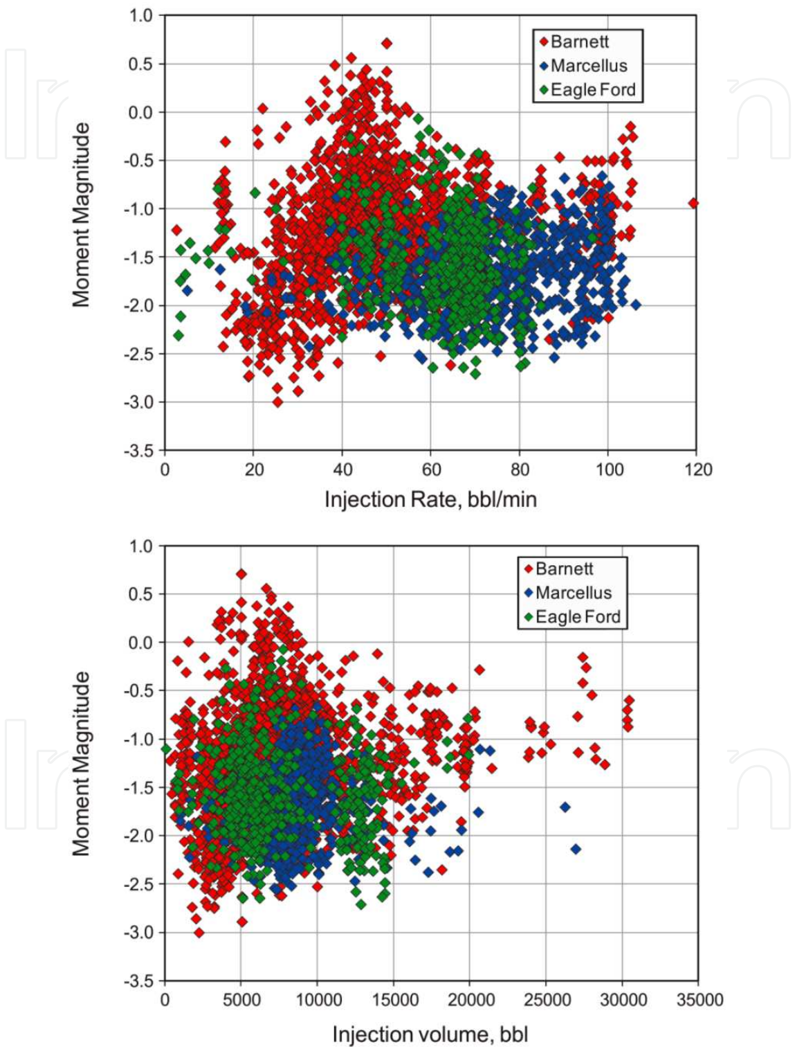
Figure 6. Effect of rate and volume on induced seismicity in three shale basins.
