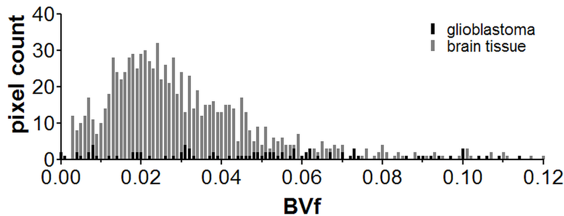
Figure 14. In humans, BVf of 1.5 to 2.0% were measured in white matter, 3.5 to 4.5% in healthy appearing gray matter and values above 6% in glioblastoma margin. Figure 14 shows the BVf distribution in a healthy brain and in a glioblastoma after correction for CA leakage.
