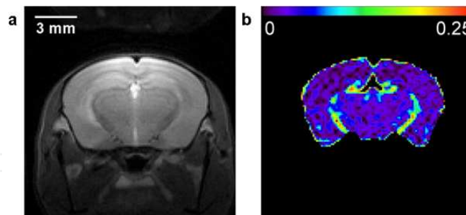
Figure 6. a: Coronal MRI image of a mouse brain showing structural details. b: Corresponding S_{\text{norm}} map showing an average cerebral BVf of 0.02 \pm 0.004 and demonstrating CA accumulation in the cerebrospinal fluid leading to overestimation of the CBV in periventricular structures.
