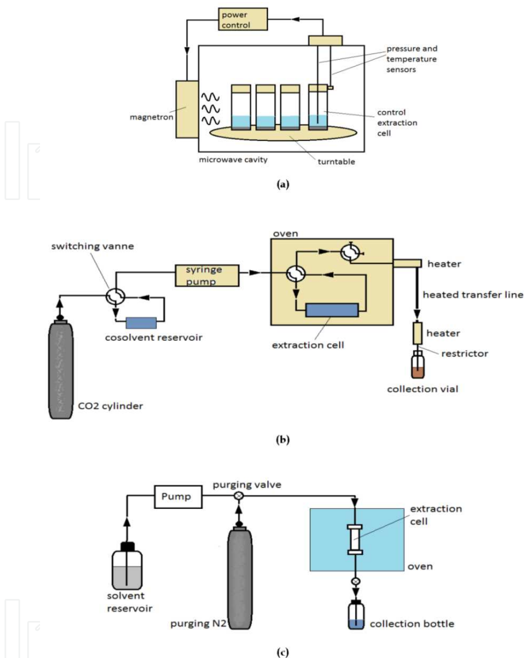
Figure 2. Extraction apparatus (a) Microwave-Assisted Extraction: MAE extraction vessels are placed on a turntable inside an oven and are subjected to microwave irradiations generated by a magnetron. A programmable microcomputer controls and monitors the power, temperature and pressure within the vessel (b) Supercritical Fluid Extraction: SFE incorporates pumps which produce the high pressures required for supercritical CO 2 work. An organic cosolvent can be added to the extraction fluid by a separate module. The extraction cell is placed in an oven which maintains a precise fluid temperature. A static mode (equilibration) and a dynamic mode (with a controlled flow-rate) can be performed successively. A restrictor valve (changing the CO 2 from condensed to gaseous phase) provides precise control over flow-rates (c) Assisted-Solvent Extraction: ASE operates by moving the extraction solvent through an extraction cell which is heated by direct contact of the oven. Extractions can be performed first in static mode; when the extraction is complete, compressed nitrogen moves the heated extracting solvent to the collection bottle.
