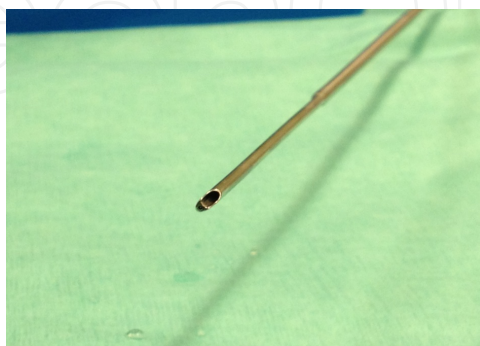
Figure 2. Distal tip of a semi-rigid ureteroscope showing the larger opening of the working channels (right side) compared to the optical opening. Note the stepped appearance as opposed to a more usually seen tapered tapered appearance. The lens is angled at 5 degrees to allow visualisation of the working instruments as they exit the channel.
