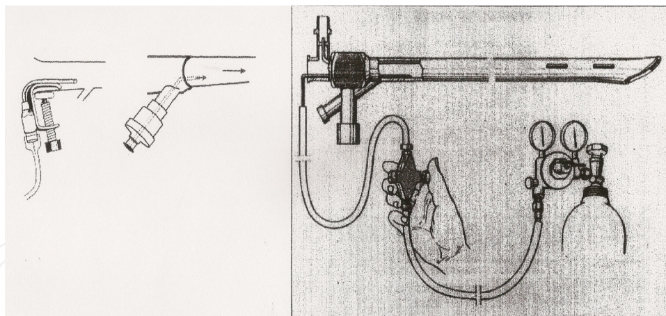
Figure 4. The injector apparatus of R. Douglas Sanders.
