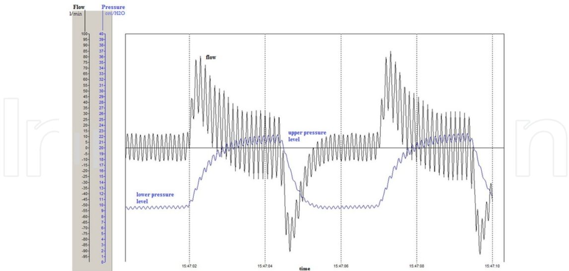
Figure 42. Characteristics of pressure and flow during ventilation with the VDR-4 ventilator. Peak airway pressure: 21 cm/H 2 O; PEEP: 9 cm/H 2 O; low-frequency: 12 cycles/min; high-frequency 500 cycles/min; inspiration:expiration ratio = 1:2.
