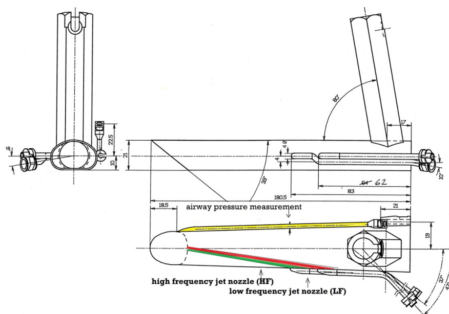
Figure 9. Schematic drawing of the gas flow in the jet laryngoscope (two jet nozzles) and of the pressure measurement and oxygen concentration ( \text{FIO}_2 ) at the tip of the endoscope (yellow nozzle).
