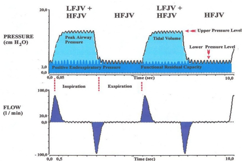
Figure 10. Relationship of pressure and flow during simultaneous low-frequency and high-frequency jet ventilation.
