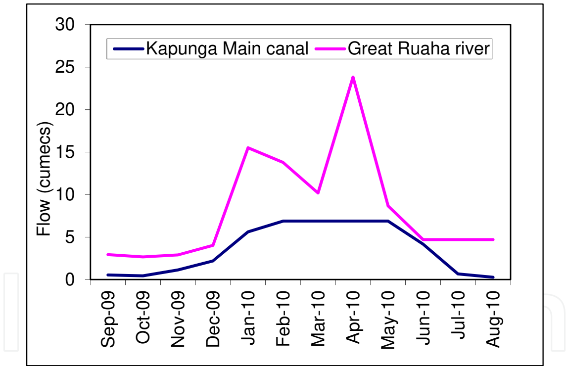
Figure 8. Seasonal hydrograph of Ruaha river and Kapunga Rice Project main canal
