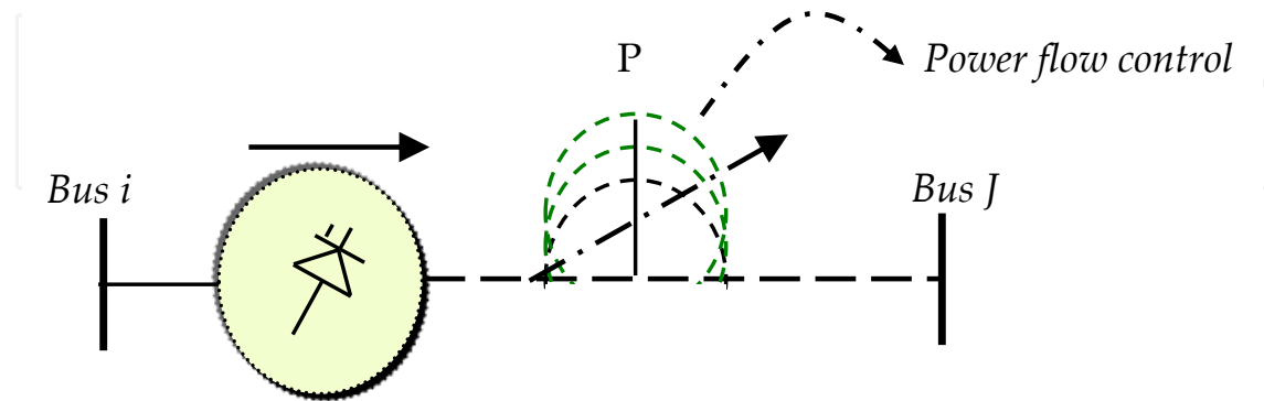
Figure 16. Series FACTS Controllers.
