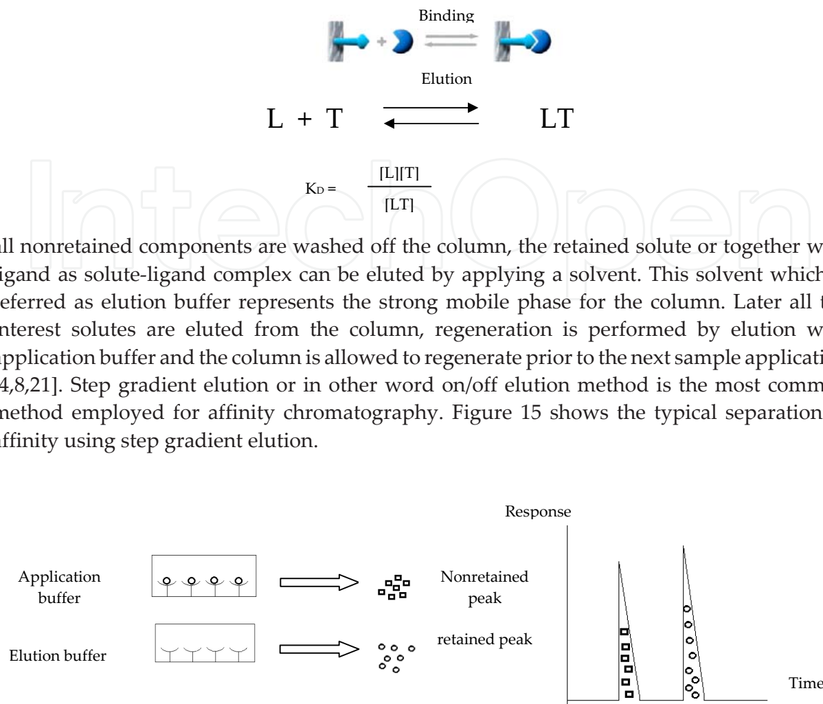
Figure 15. Typical separation in affinity using step gradient elution.
