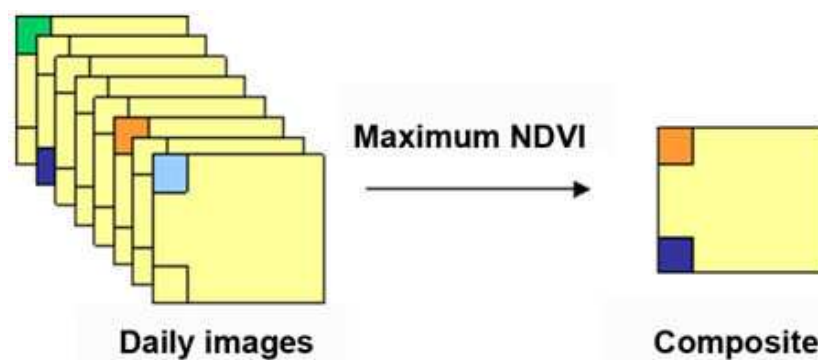
Figure 2. Maximum NDVI standard compositing
