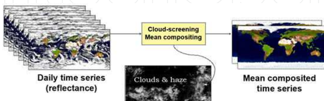
Figure 3. Mean compositing method
