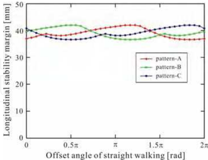
Figure 7. Result of longitudinal stability margin
