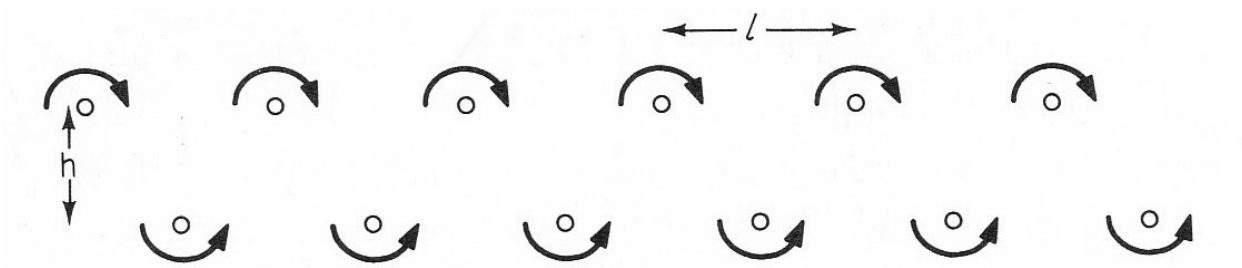
Figure 7. Von Karman vortex streets.
