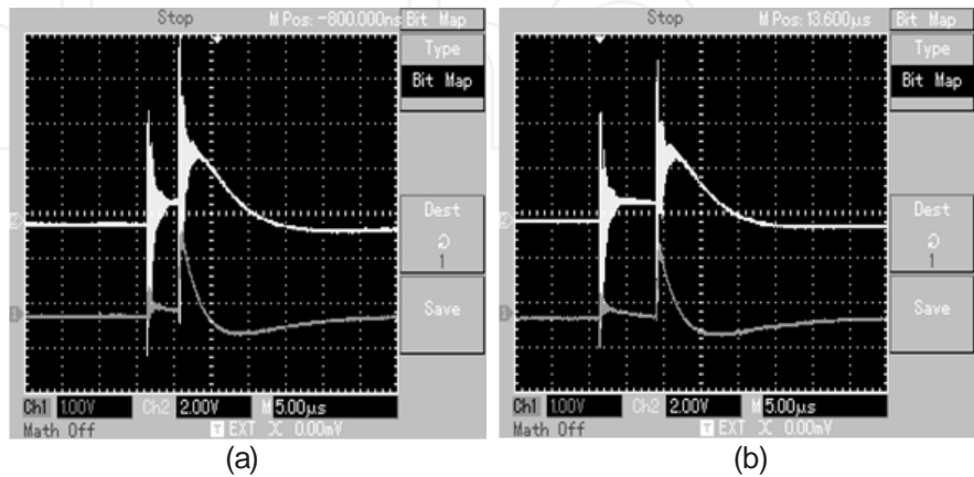
Figure 18. Oscillograms of the discharge current (top curve) and signal piezo-ceramic pressure sensor (lower curve): a) d = 0.5 mm, b) d = 1 mm. Tap water flow = 15\text{ cm}^3/\text{sec} , without the input gas stream, C = 0.18\text{ }\mu\text{F} , U = 13.5\text{ kV} ; ballast resistor in the discharge circle: R_b = 20\text{ }\Omega , the cylinder is in horizontal position.
