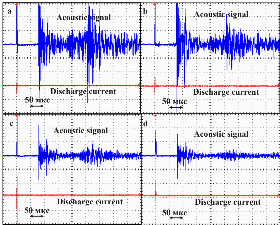
Figure 19. Oscillograms of current and acoustic signal in the single pulse mode at the different discharge ballast resistor: R_b : a) - 0\text{ }\Omega , b) - 10\text{ }\Omega , c) - 20\text{ }\Omega , d) - 50\text{ }\Omega . Tap water flow 15\text{ cm}^3/\text{s} , without the input gas stream, d = 0.5\text{ mm} , C = 0.015\text{ }\mu\text{F} , U = 19.5\text{ kV} , the cylinder is in horizontal position.
