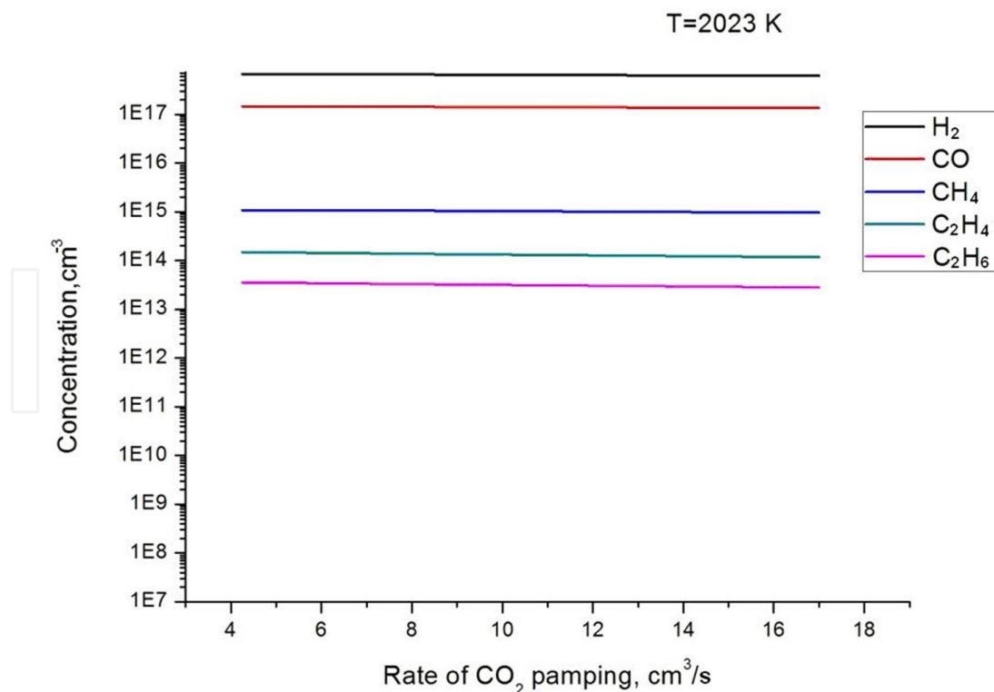
Figure 11. The dependence of the reaction main products of the flow rate of CO_2 (inside discharge), T = 2023\text{ K}
