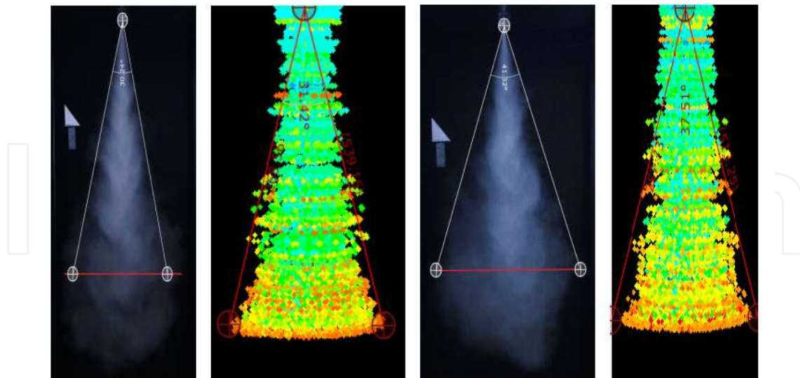
Figure 11. B100 (left) is 30.24° (experiment), 31.42° (simulation) and D100 (right) is 41.32° (experiment), 37.51° (simulation) at 0.2 MPa
