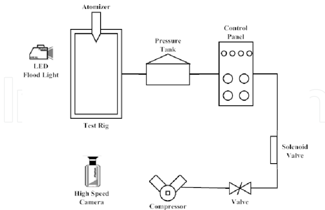
Figure 3. Experimental testing set up
