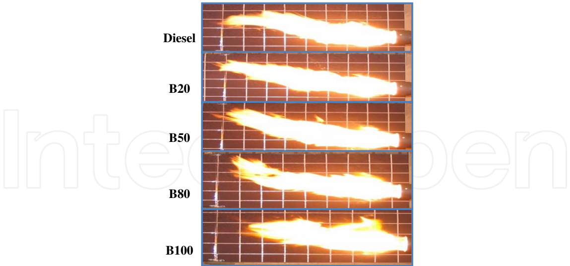
Figure 17. Open fire testing for five type of fuel
