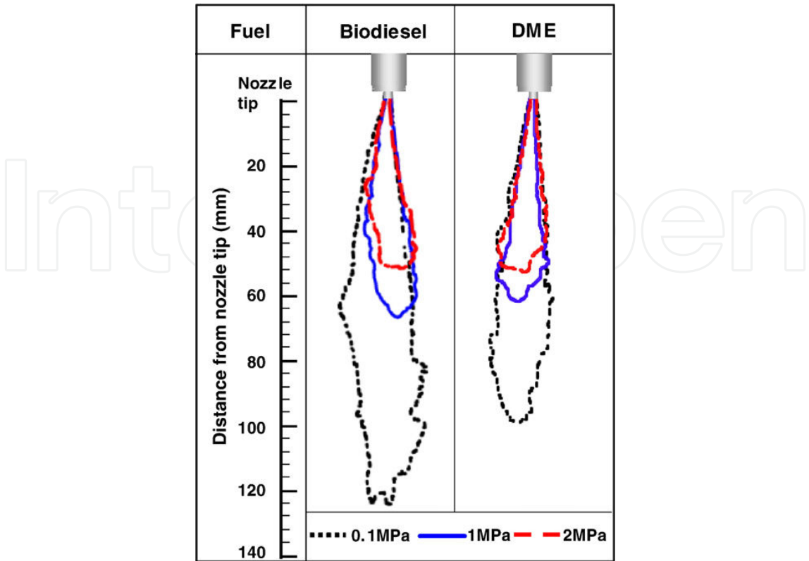
Figure 6. Spray length and spray pattern for different injection pressure
