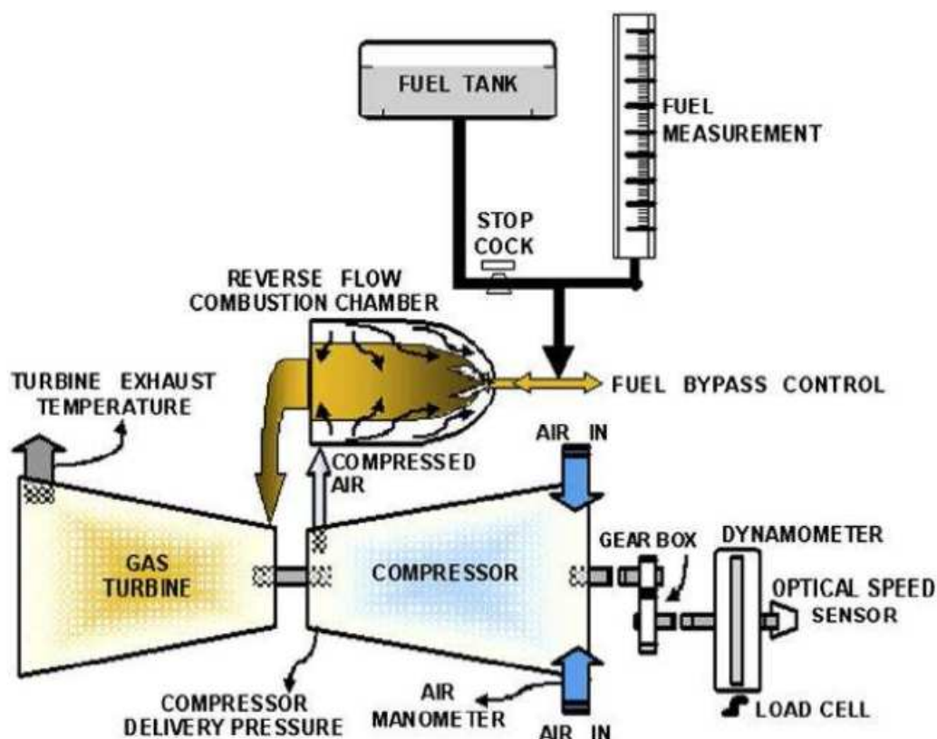
Figure 2. Simple actual flow in gas turbine
