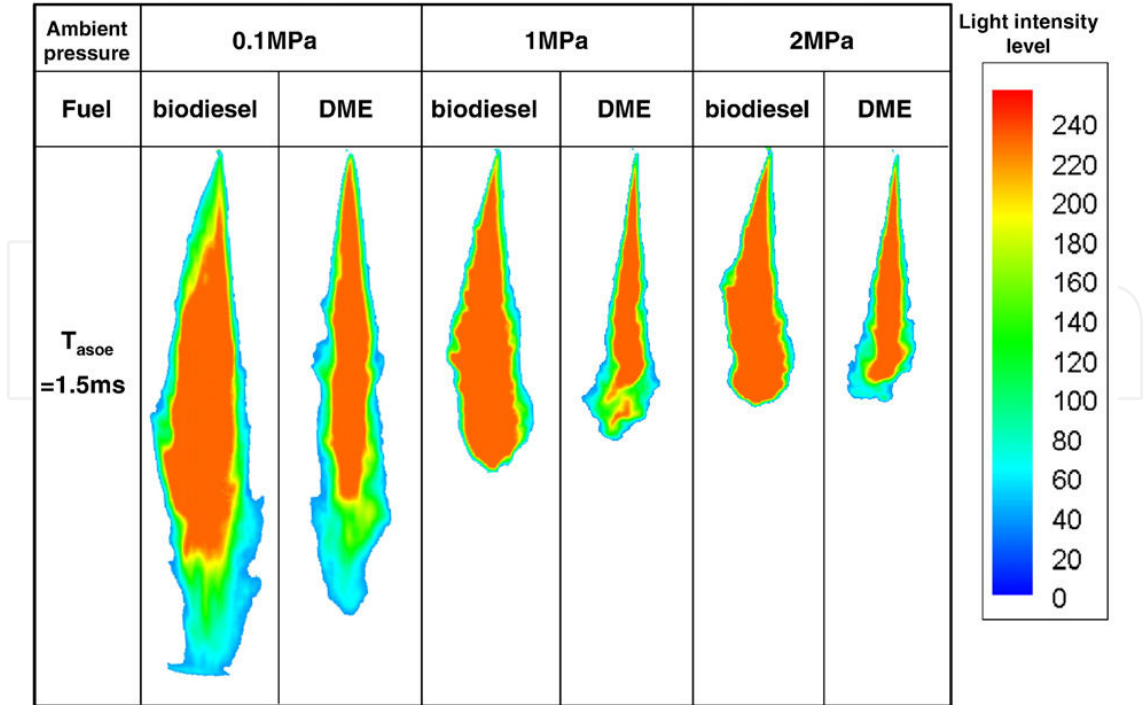
Figure 7. The contour plot of biodiesel and DME fuels at various ambient pressures
