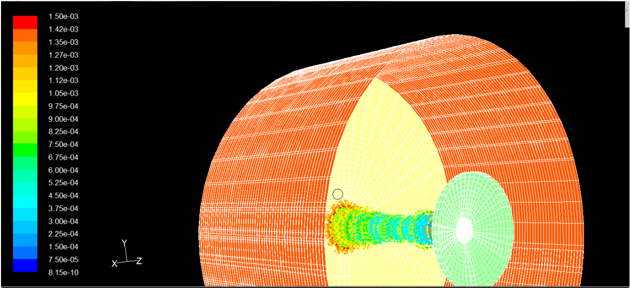
Figure 9. Domain of the spray
