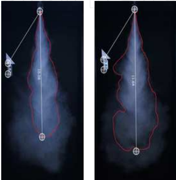
Figure 13. D100 (left) and B100 (right) at 0.2 Mpa
