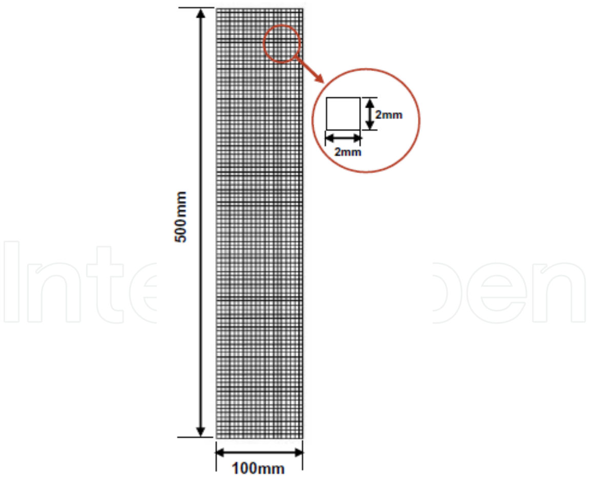
Figure 5. Computational grid for the numerical analysis
