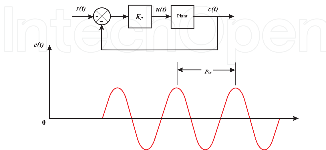
Figure 11. Second tuning method of Ziegler-Nicholds.
