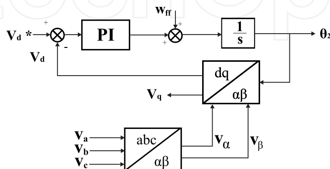
Figure 15. PLL synchronous reference frame
