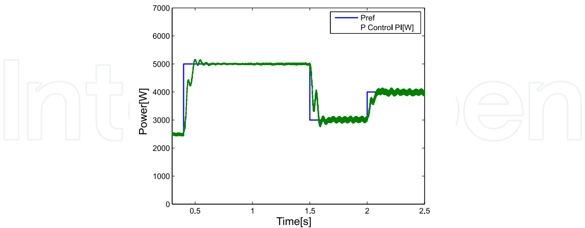
Figure 21. Power generated by SRG and the reference power.
