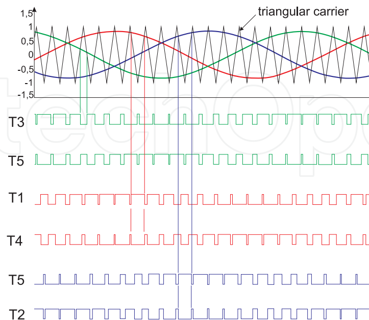
Figure 13. Modulation PWM sinusoidal
