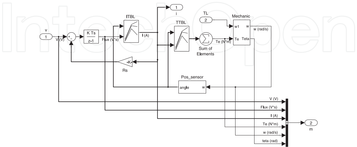
Figure 20. Diagram SRM model in Simulink.
