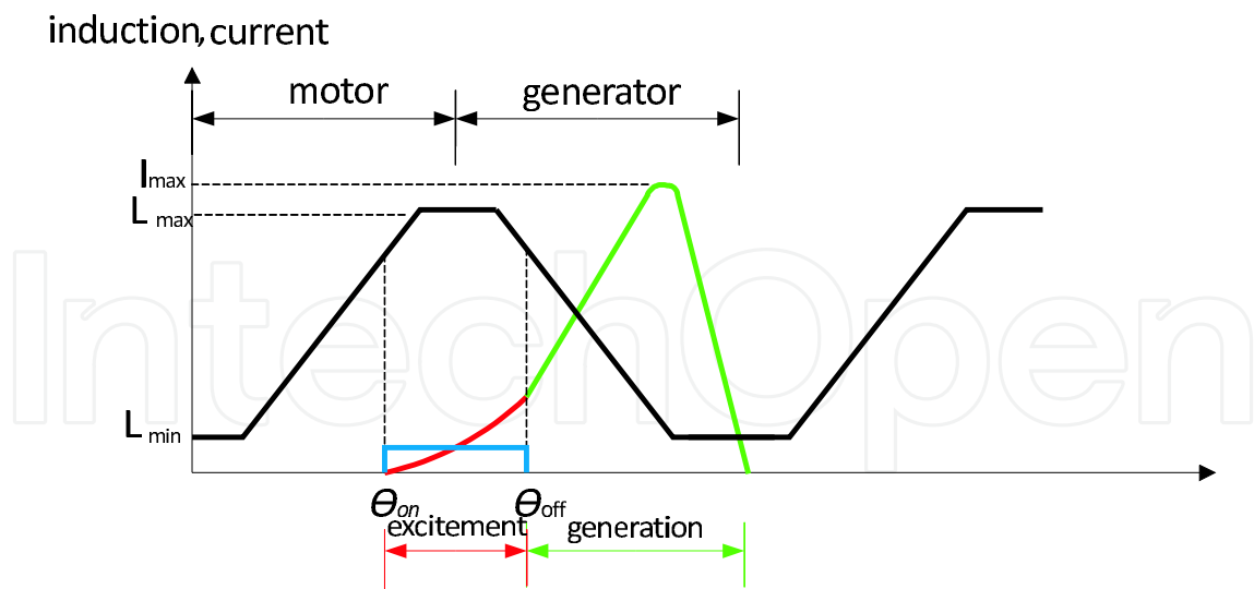
Figure 4. Profile of the Inductance..
