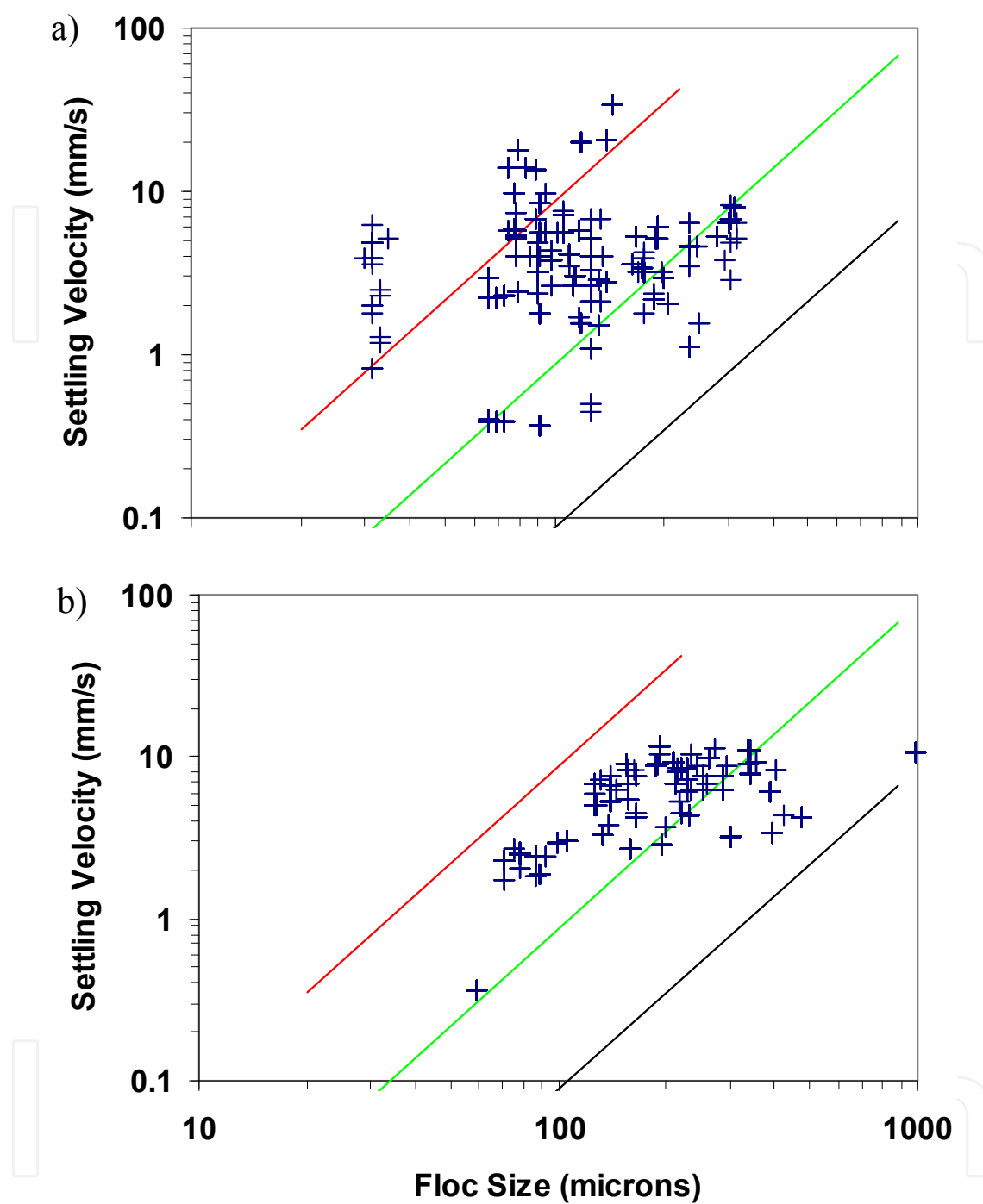
Figure 10. Settling settling vs. floc size for Portsmouth Harbour samples: a) 4_A (38M:62S); b) 6_B (38M:62S). Both samples had nominal 2 g.l -1 total SPM concentrations and were sheared at a stress of 0.35 Pa. Diagonal lines represent contours of constant Stokes equivalent effective density: red = 1600 kgm -3 , green = 160 kgm -3 , and black = 16 kgm -3 .
