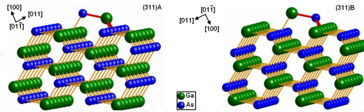
Figure 14. The surface structures of GaAs(311)A (left figure) and (311)B (right figure) substrates. Green balls are Ga atoms, blue balls are As atoms, and yellow and red sticks are Ga-As bonds.
