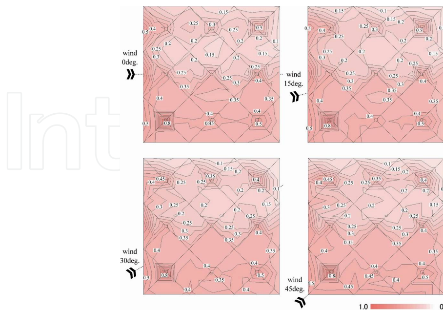
Figure 24. Fluctuating wind pressure coefficient which were obtained from wind tunnel tests on open type of the multi-bay mode
