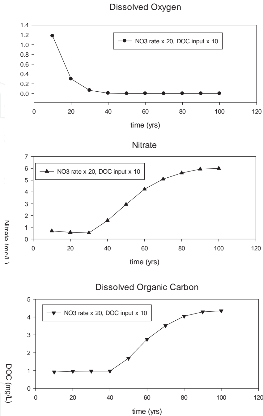
Figure 7. Simulated concentration changes of dissolved oxygen, nitrate, and DOC at the San Joaquin River discharge area assuming the nitrate V_{\max} is increased by a factor of 20 and DOC concentrations in recharge are increased to 10 mg/L.
