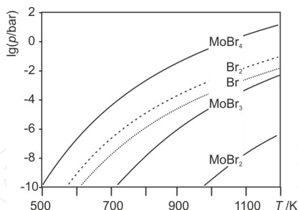
Figure 5. Composition of the gas phase for the auto transport of \text{MoBr}_3 .
