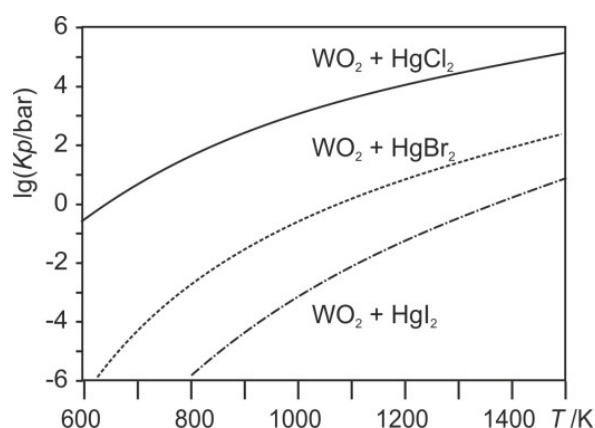
Figure 11. Equilibrium constants of transport reactions of \text{WO}_2(s) with \text{HgX}_2(g) , X = \text{Cl}, \text{Br}, \text{I} .
