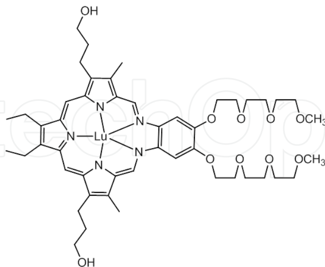
Figure 23. Structure of Lu-texaphyrin (PCI-0123).
