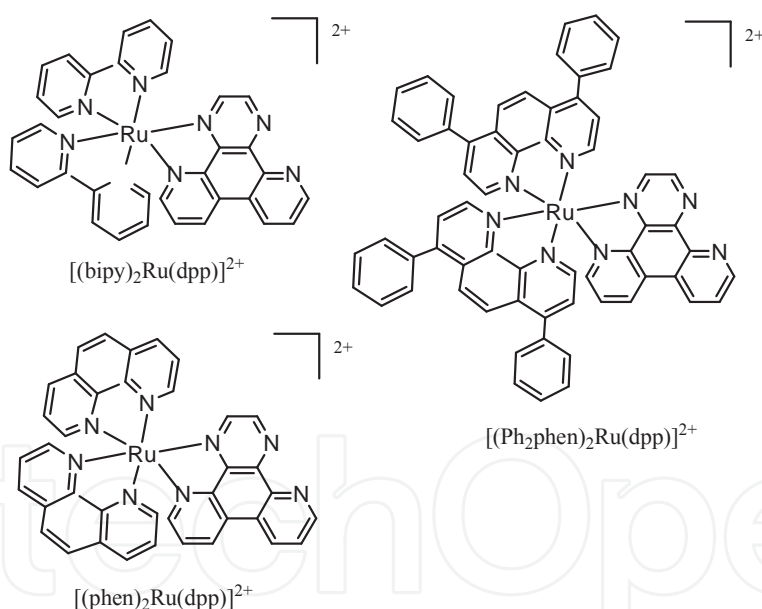
Figure 12. DNA photocleavage agents [(\text{TL})_2\text{Ru}(\text{dpp})]\text{Cl}_2 with TL = 2,2'-bipyridine (bpy), 1,10-phenanthroline (phen) or 4,7-diphenyl-1,10-phenanthroline (Ph 2 phen), with the polyazine bridging ligand 2,3-bis(2-pyridyl)pyrazine (dpp).
