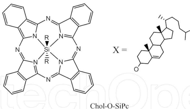
Figure 18. Structure of bis(cholesteryloxy) derivative of SiPc.
