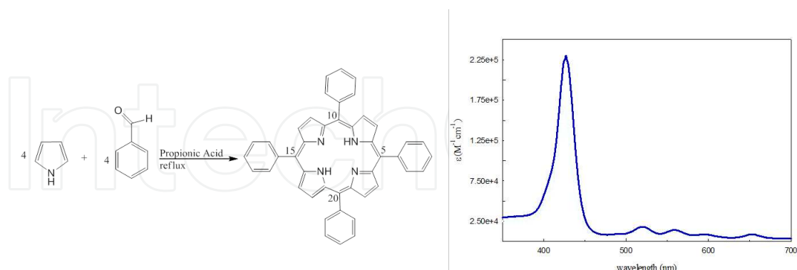
Figure 4. Synthesis and electronic spectra of meso -tetraphenylporphyrin (H 2 TPP).
