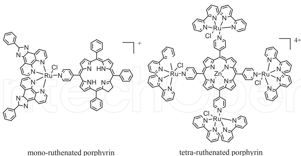
Figure 13. The structure of the mono-ruthenated porphyrin: [MPyTPPARu(pip)2Cl] + and the structure of tetra-ruthenated porphyrin: μ-{meso-5,10,15,20-tetra(4-pyridyl)porphyrin}-tetrakis-{bis-(bipyridine)chlororuthenium(II)} 4+ .
