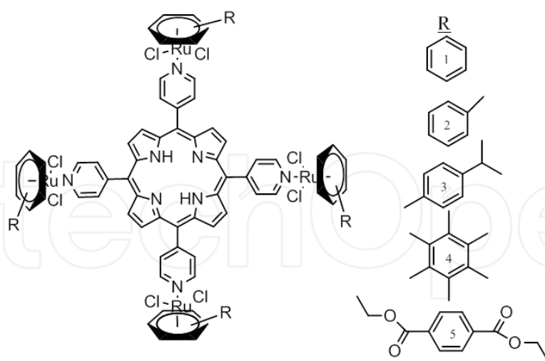
Figure 14. Structures of ruthenated tetraphenyl porphyrins.
