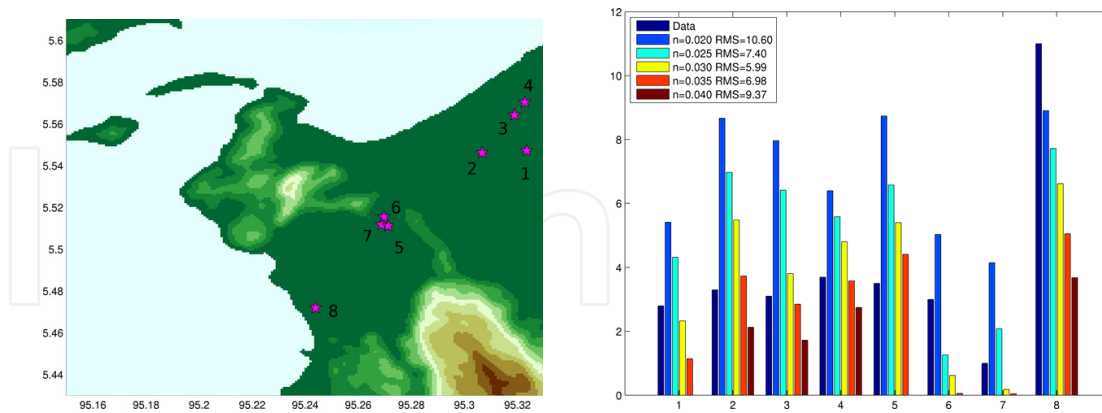
Figure 11. a) Positions of field measurements, b) model results for varying roughness parameters in comparison.
