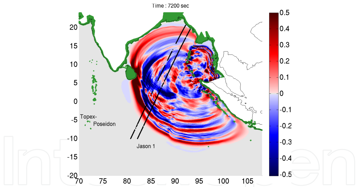
Figure 8. Model snapshot after two hours. Sea surface elevation together with the positions of the satellite tracks Jason 1 and TOPEX/POSEIDON
