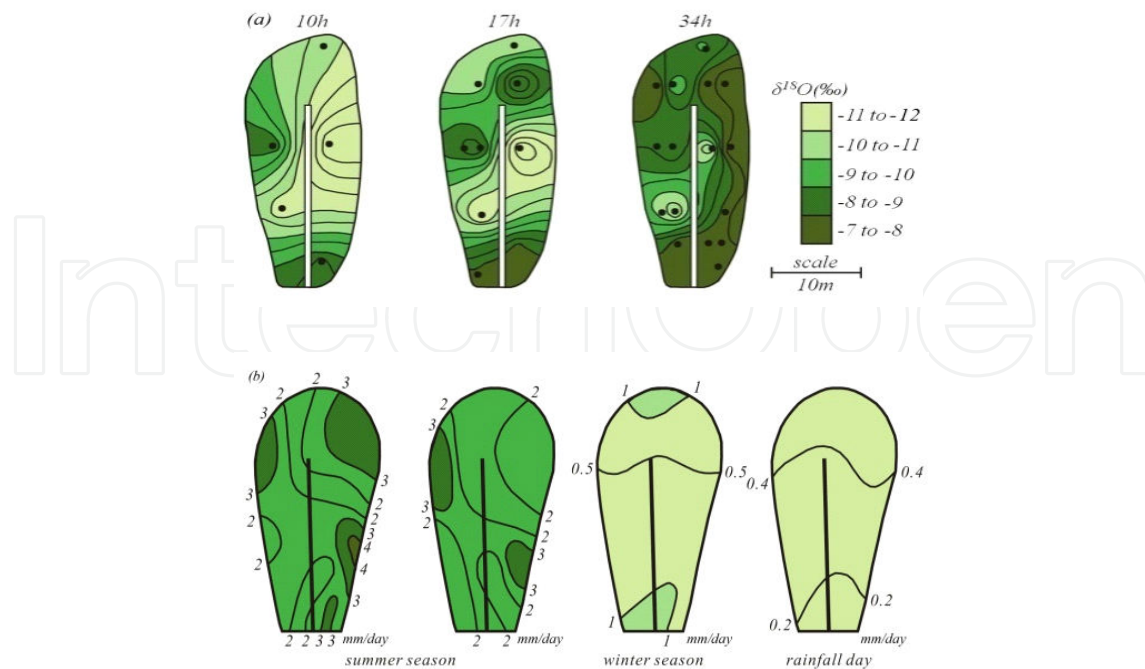
Figure 15. (a) Contour diagrams of \delta^{18}O in groundwater at three sampling times and (b) Typical spatial distribution of the daily land evaporation rate.
