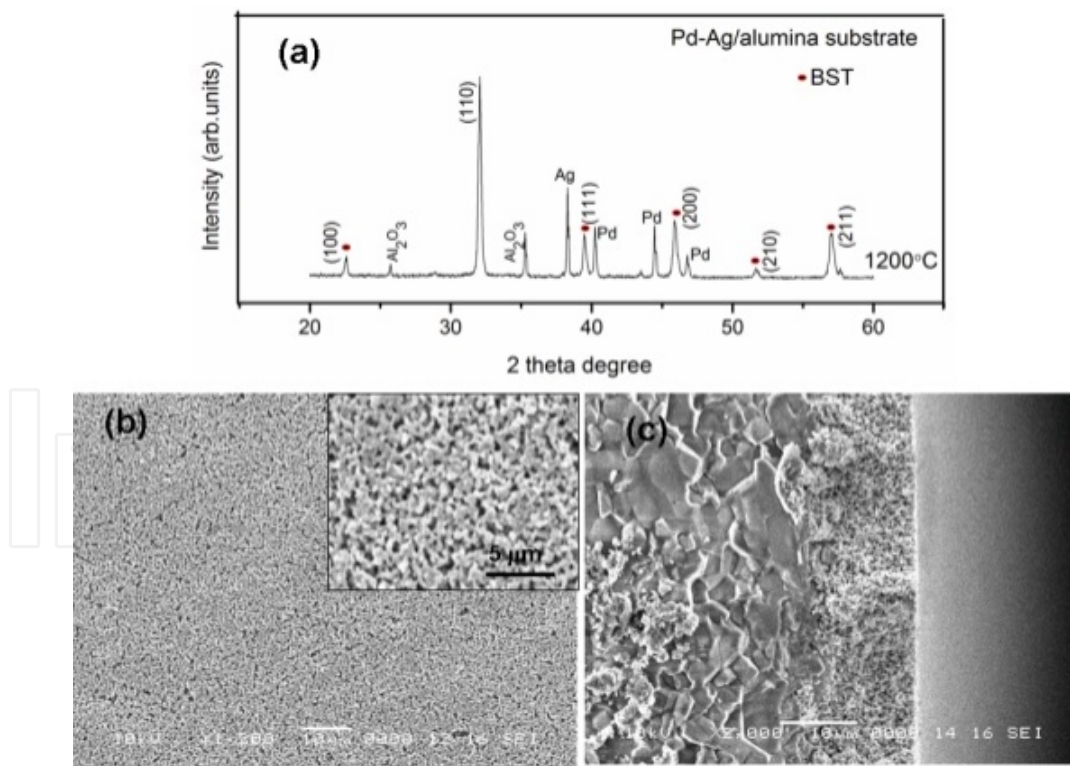
Figure 14. The BST thick films deposited on Pd-Ag/alumina substrate by screen-printing sintered at 1200°C: (a) the XRD pattern; (b) the surface, together with (c) the cross-section micrographs indicating the thickness of about 10 \mu\text{m} . Inset shows the magnified surface picture.
