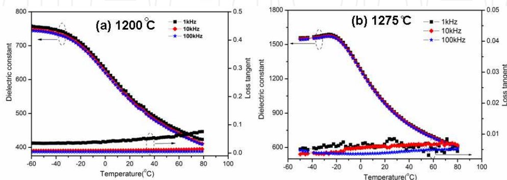
Figure 8. Temperature dependences of dielectric constant and loss tangent for the BST-MgO ceramics sintered at 1200 and 1275°C via hybrid process.
