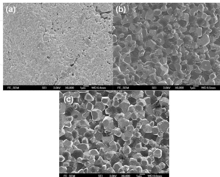
Figure 7. The surface morphologies of BST composite bulk ceramics sintered at (a) 1200°C ; (b) 1275°C; (b) 1300°C for 2 h via the hybrid process. Note: the EDX results suggested that grains with light color corresponded to the BST phase while grains with dark color were MgO phase.
