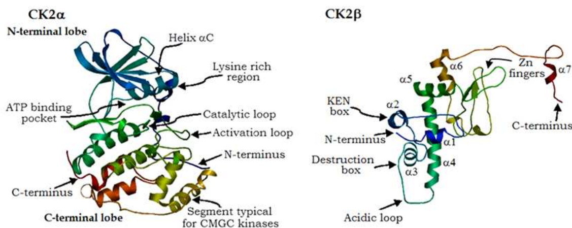
Fig. 1. Model structures of the CK2 \alpha and CK2 \beta subunits from Mytilus galloprovincialis (Mediterranean mussel) (Kouyounou-Koutsoukou et al., 2011b)
