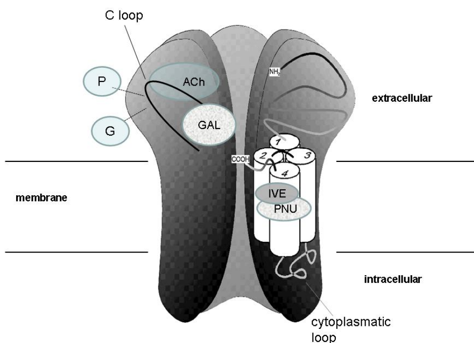
Fig. 1. Schematic representation of a nicotinic Acetylcholine Receptor (nAChR)
