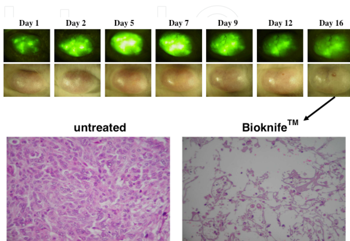
Figure 6. A time-course analysis of BioKnife™ infection of subcutaneously inoculated PC3 tumor cells in a nude mouse. Photomicrographs of tissue specimens on day 16 are presented in the bottom two panels.
