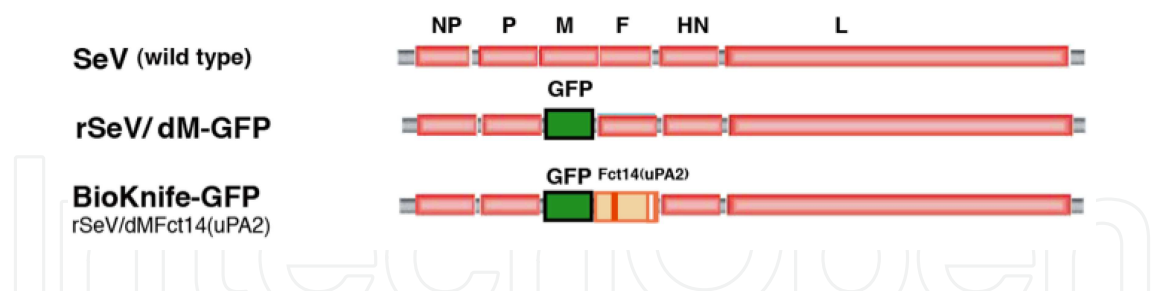
Figure 5. Gene structure of recombinant SeV. Wild type SeV is pictured at the top of the figure, which is followed by the M-gene deleted SeV with a substitutive load of the Green fluorescent protein (GFP) gene (rSeV/dM-GFP) in the middle. Finally, at the bottom, the F gene of rSeV/dM-GFP is transformed to a uPA-sensitive sequence (BioKnife™-GFP).
