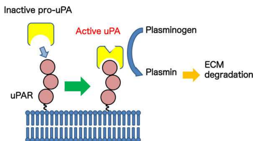
Figure 3. Schematic model of the urokinase activation system.
