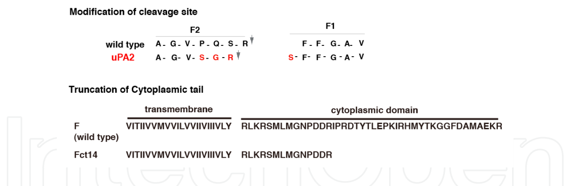
Figure 4. Modification of the cleavage site of the SeV-F protein, which is sensitive to the urokinase-type plasminogen activator, and truncation of the cytoplasmic tail resulted in optimization of the cell-fusion activity.
